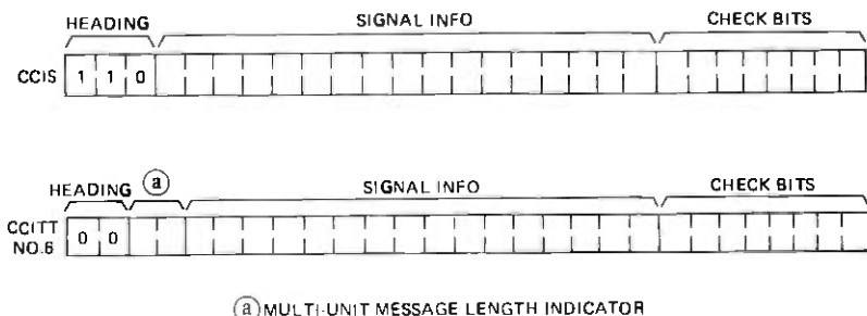
Fig. 9—Subsequent Signal Unit (SSU) format.
