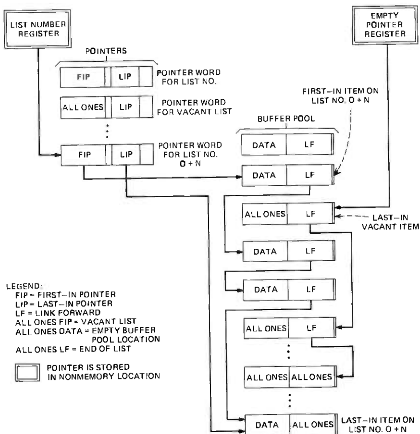
Fig. 16—List linkages.
