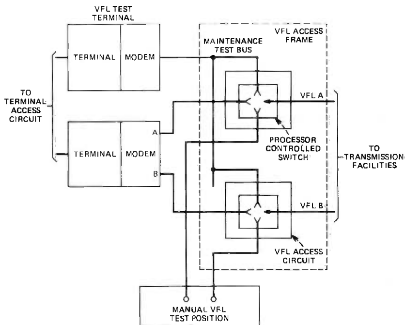
Fig. 2—STP VFL arrangement and dual VFL configuration.
