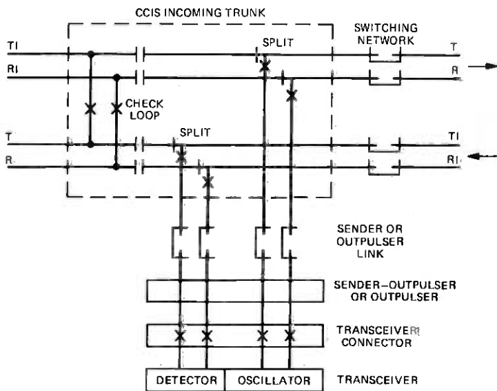
Fig. 3—Continuity check.
