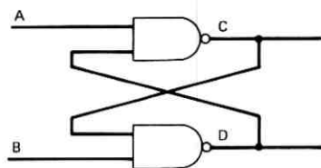
Fig. 2—NAND flip-flop.
