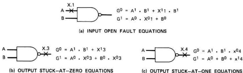
Fig. 8—Equations for handling faults in combinational circuits.
