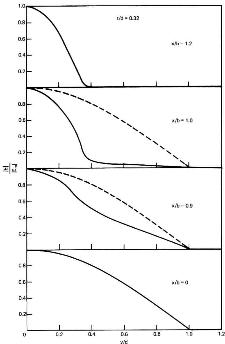
Fig. 4—Magnitude of the electric field vector relative to its maximum value at y = 0 as a function of the normalized vertical dimension y/d . Solid and broken curves describe the single-material fiber with t/d = 0.32 and t/d = 0 .
