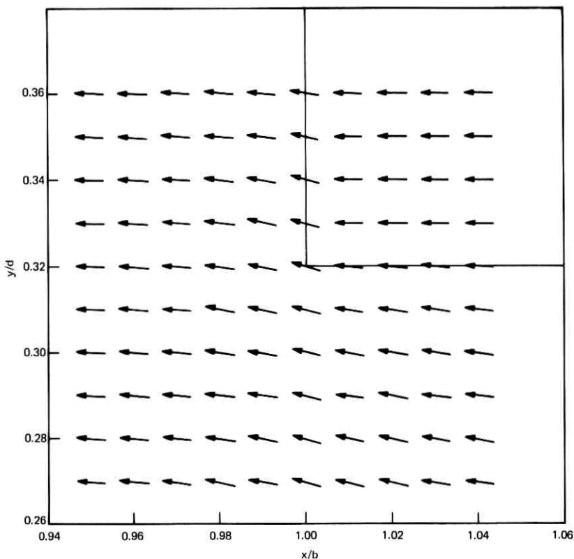
Fig. 9—Short arrows indicate the direction of the electric field vector of the lowest-order mode of the single-material fiber, with t/d = 0.32 near the corner of the dielectric material where the support slab is attached to the core.
