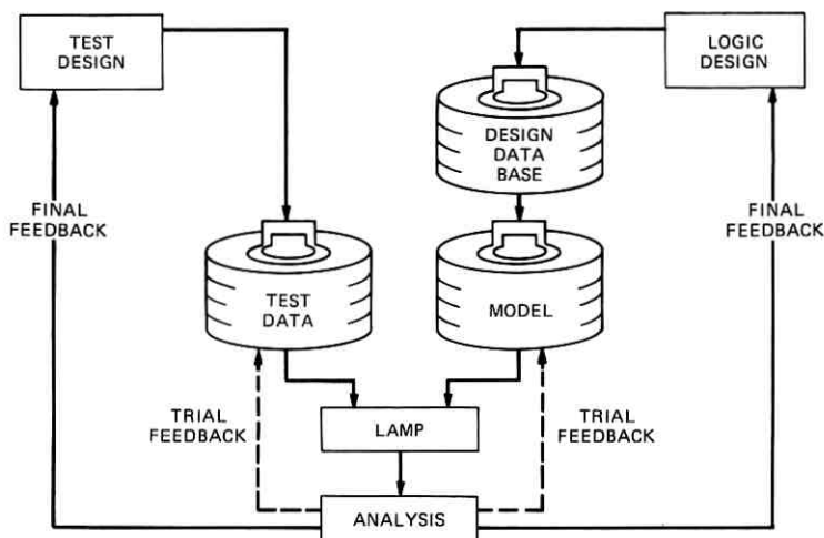
Fig. 1—Design verification.
