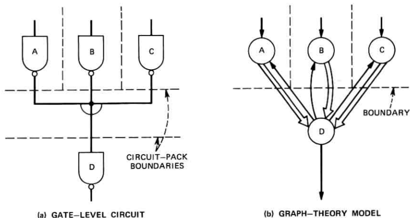
Fig. 11—Collector-tie considerations.
