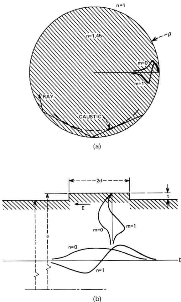
Fig. 2—(a) Whispering-gallery modes clinging to a circular boundary with effective radius \rho (= a/\sin^2 \theta) . The field ( m = 0, 1, \dots ) is described exactly by Bessel functions and approximately by Airy functions. (b) Cross section in a local r, \xi plane.
