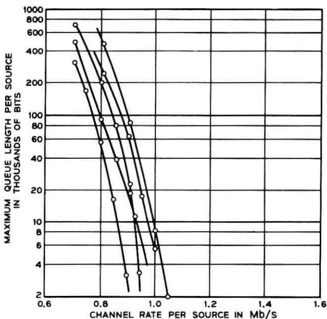
Fig. 24—Buffer requirements versus channel rate when data from twelve sources is combined prior to transmission.
