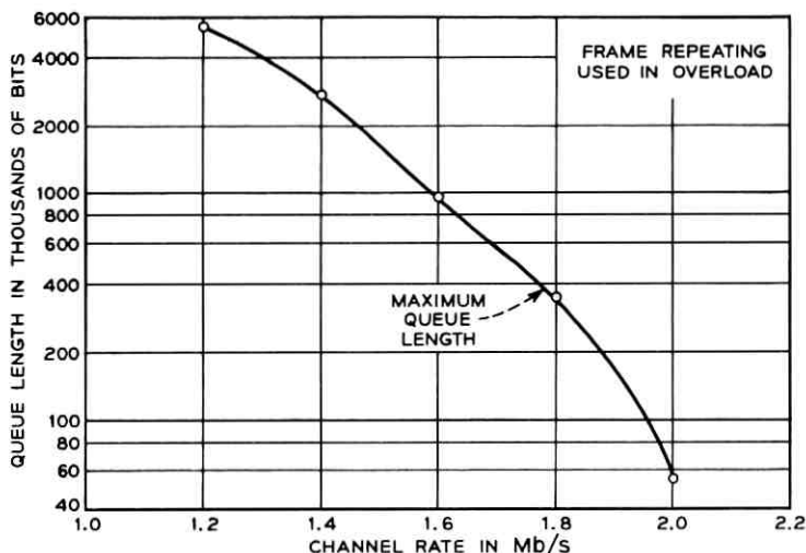
Fig. 14—Buffer requirements versus channel rate for a single source and 0.11-percent probability of overload. Overload detected via queue length in present field. (Curve is very close to that of Fig. 13.)
