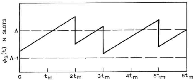
Fig. 2—A typical graph of the output of the phase comparator.
