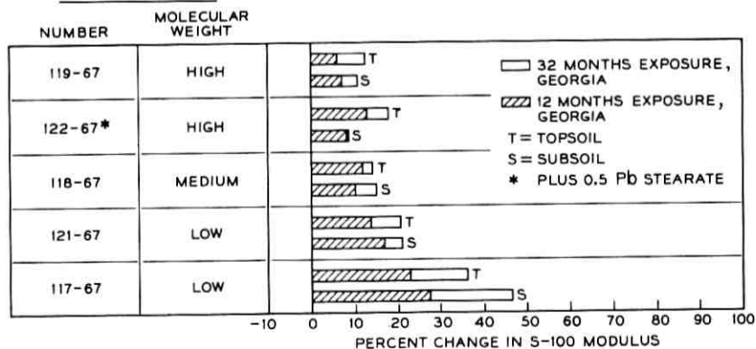
Fig. 10—Effect of soil burial on the modulus of sheet vinyls containing polyester plasticizers.
