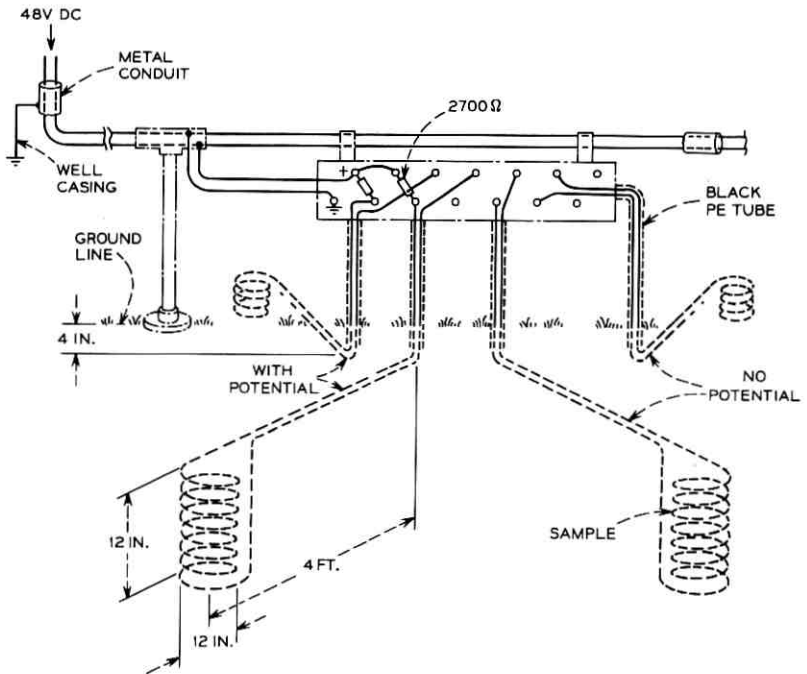
Fig. 13—Method of exposure for insulated wire samples.
