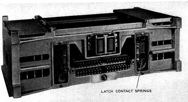
Fig. 32 — Jack side of dynamic unit showing latch contact springs.
