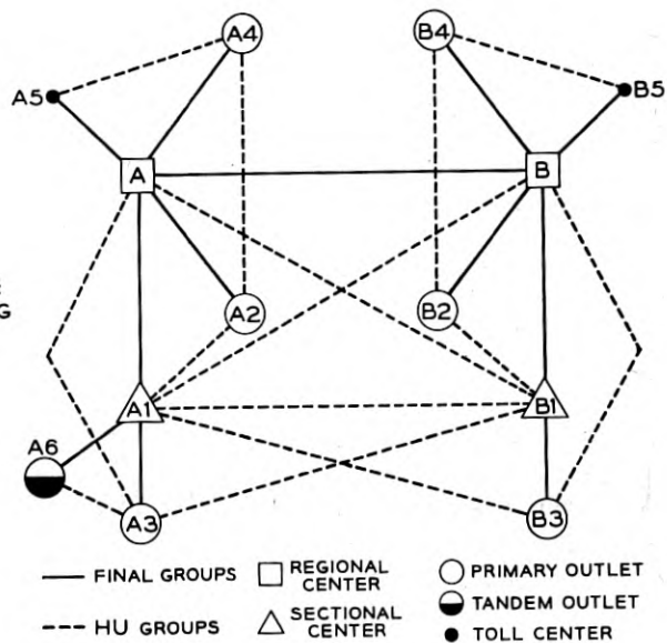
Fig. 1 — Typical intertoll trunk networks.
