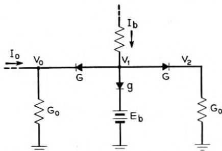
Fig. 5 — Transmission type diode gate.
