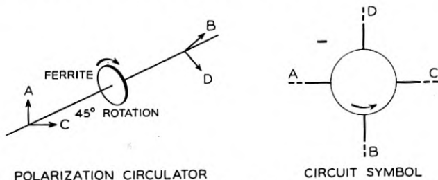
Fig. 9 — Schematic representation of polarization circulator. The ferrite is adjusted to 45^\circ rotation by an external field, not shown. The circuit symbol for the circulator is shown at the right.
