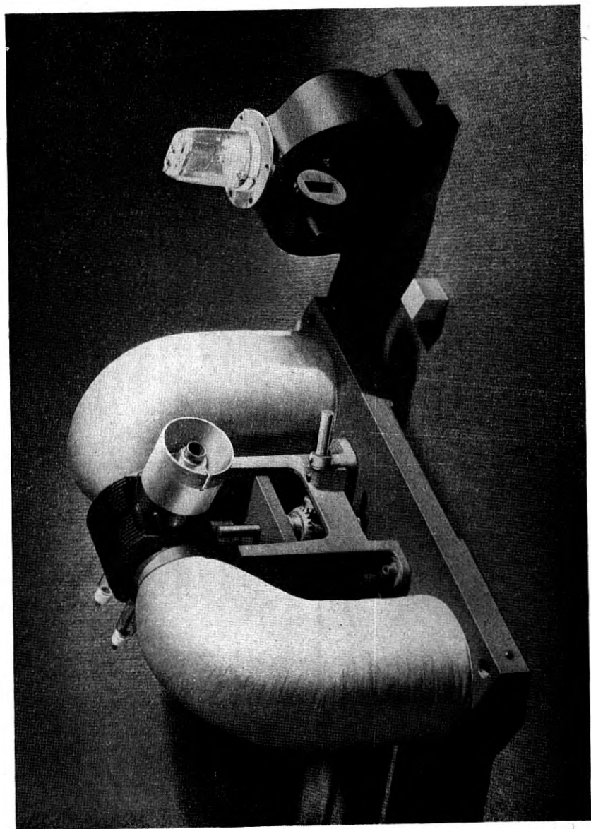
Fig. 44—The 720A-E (1000 mc/s, \sim 2800 kw., \sim 2800 mc/s) and the 725A (55 kw., 9375 mc/s) magnetrons, shown at the left and right respectively, each mounted in its magnet.
