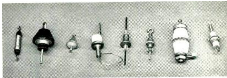
Fig. 3—An array of similar sizes of terminals. From left, they are: rubber-sealed, molded phenolic-sealed, glass-sealed, copper-glass, fluorocarbon resin-sealed, molded plastic-sealed, gasket-sealed ceramic, and solder-sealed high alumina ceramic.
