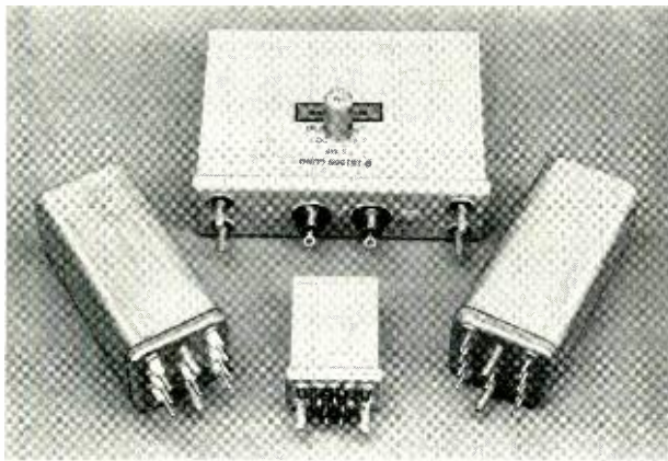
Fig. 1— Apparatus cans using various types of sealed terminals: left, solder-sealed ceramic; center foreground, rubber-sealed; center, molded phenolic; and right, glass-sealed. The small tubular can atop the large unit, center, shows the use of cold-compression fluorocarbon resin-sealed terminals.
