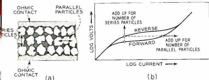
Fig. 3 — Simplified cross-section of a silicon carbide varistor (a) and a voltage-current characteristic of a contact to a single particle (b).
