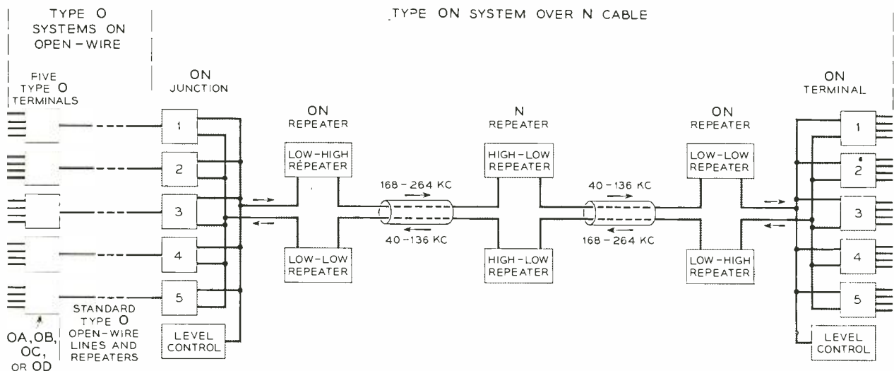
Fig. 3 — Typical Type-ON system on open-wire and cable.
