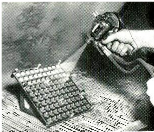
Fig. 6 — Metallizing gun in operation for applying electrodes of copper or tin to varistors.
