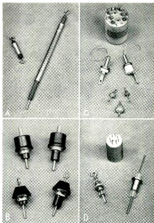
Fig. 2— A, large and small rubber-sealed terminals. B, short-shank (left) and long-shank molded phenolic terminals. C, copper-glass (center) and examples of glass-sealed terminals. D, molded plastic (left) and examples of cold-compression fluorocarbon resin-sealed terminals.
