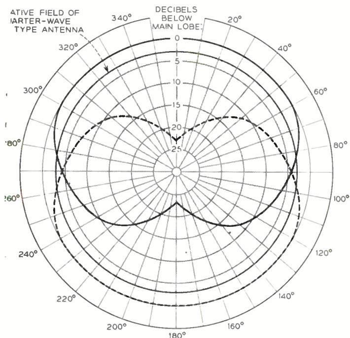
Fig. 3 — Pattern for switchable mobile antenna.
