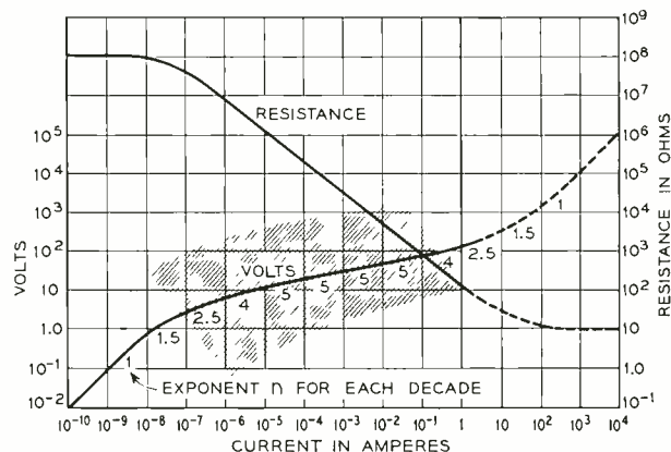
Fig. 1 — Typical characteristics of a silicon carbide varistor relating voltage and resistance to current.
