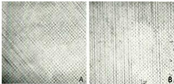
Fig. 2 — Slip lines on an exposed surface of (A) crystal compressed at 525°C and (B) crystal twisted at 600°C. Magnification 75 diameters.
