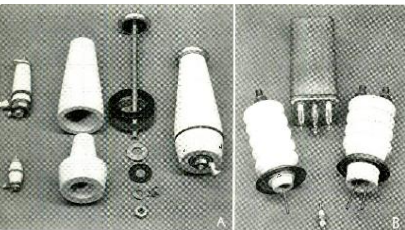
Fig. 4 — A, three sizes of gasket-sealed ceramic terminals with a large terminal disassembled. The terminal at upper left contains two coaxial feed-throughs. B, examples of solder-sealed high alumina ceramic terminals.
