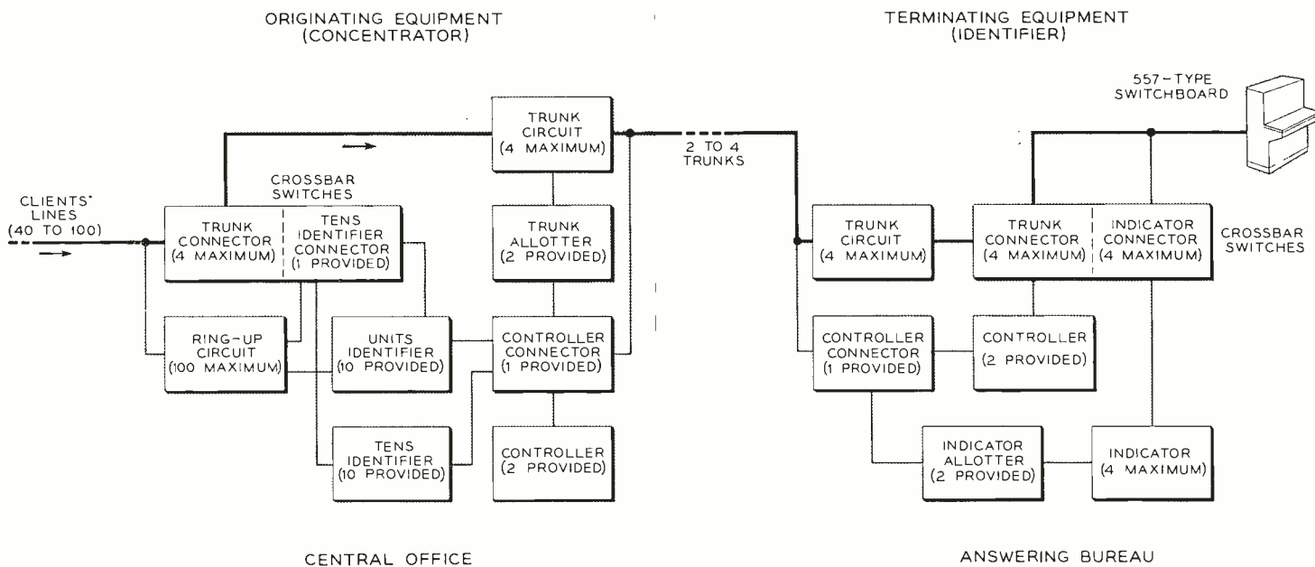
Fig. 1 — Block diagram of concentrator-identifier arrangement.
