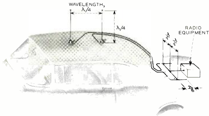
Fig. 2 — Mobile unit equipped with a switchable antenna.
