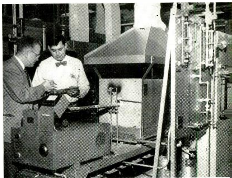
Fig. 4 — Varistor discs are placed on "boats" to travel through the furnace. Discs are fired for about one hour. The author (left) inspects a "boat" that is held by M. D. Patterson.
