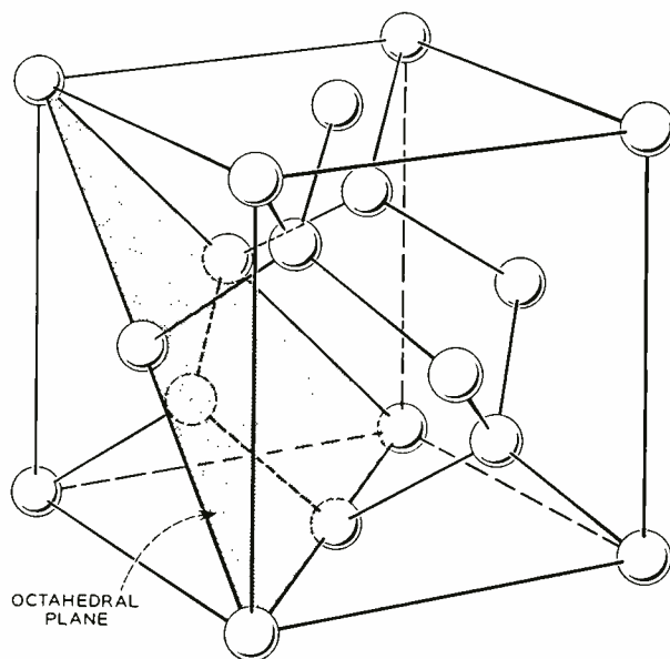
Fig. 3 — The unit cell of germanium. One of the octahedral planes, a slip plane, is cross hatched. Length of the cube edge is 5.658 angstroms (0.05658 millionths of a centimeter).
