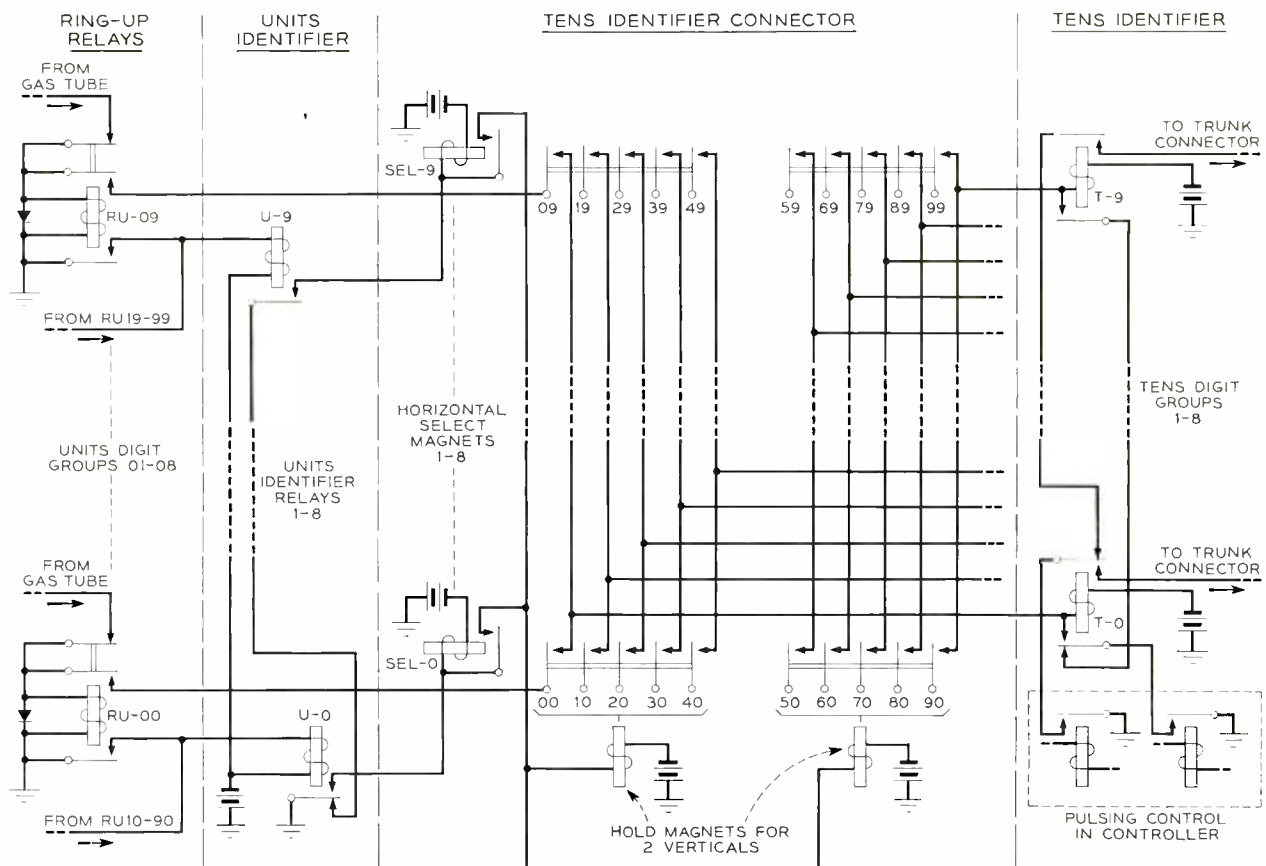
Fig. 4 — Basic plan of concentrator line-identification equipment.
