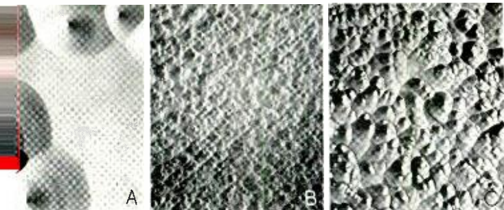
Fig. 4—Dislocation pit patterns in a germanium crystal on an octahedral face magnified 325 diameters. A—As grown—density is 60,000 per square centimeter. B—After compression of 2.5 per cent at 625°C. Density is 15,000,000 per square centimeter. C—After compression and thermal treatment at 825°C for 24 hours. Density is 3,000,000 per square centimeter.
