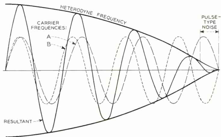
Fig. 4 — Heterodyning effect of two sine waves.
