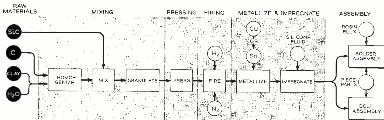
Fig. 5 — Flow chart of process for fabricating silicon carbide varistors.
