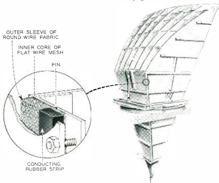
Fig. 1—Horn-reflector antenna showing details of combination seal and installation in seam.
