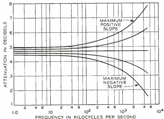
Fig. 4 — Several typical loss characteristics of one of the adjustable equalizers for A2A.
