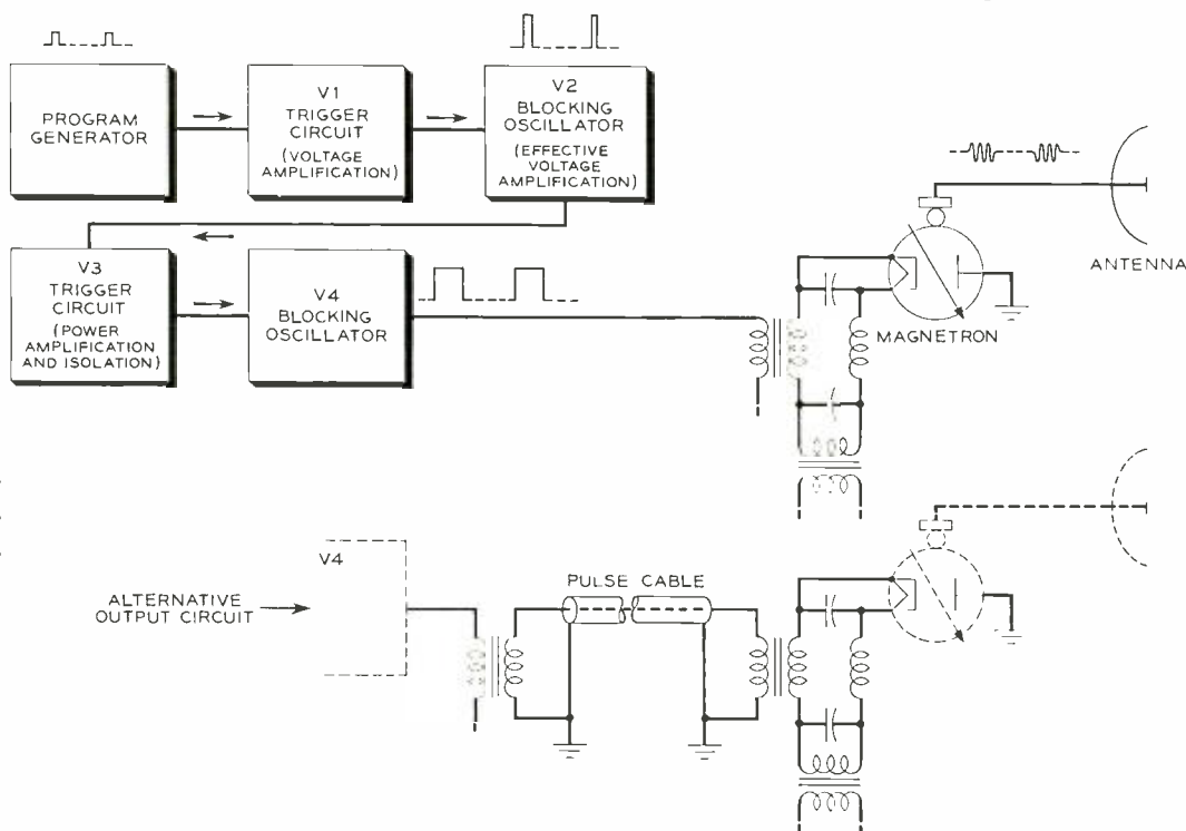
Fig. 5—Block diagram of more complex circuit required for accurately controlled pulses.
