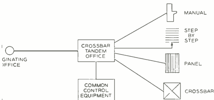
Fig. 3—Common-control equipment in crossbar tandem permits outpulsing to several types of offices.
