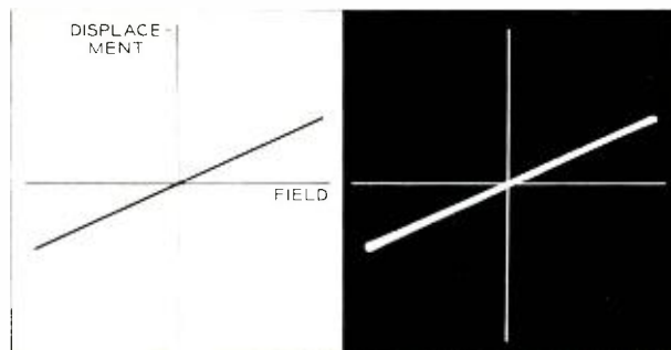
Fig. 1—A voltage applied to a crystal produces in it an electric field measured by the ratio of the voltage to the separation of the electrodes. In almost all crystals an electric field produces a proportional displacement of electric charge. The constant of proportionality is the dielectric permittivity. The dielectric constant is the ratio of that permittivity to the permittivity of empty space.
