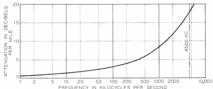
Fig. 2 — Attenuation characteristic of cable used.
