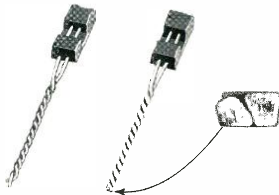
Fig. 4 — Twin wires: (left) twisted only; and (right) twisted, swaged, and trimmed.
