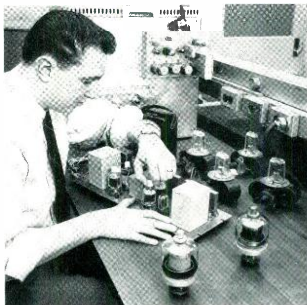
Fig. 4 — H. J. Betzel attaching plate lead to pulser tube. In higher power circuits, magnetrons (shown in the background) are pulsed by larger hard tubes (shown in the foreground).
