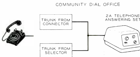
Fig. 4—A 7A announcement system uses a 2A answering machine as in the headpiece illustration.
