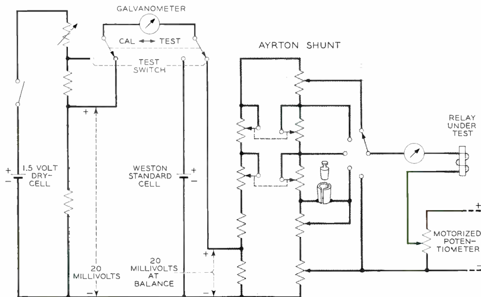
Fig. 1 — When the relay test current is of the desired value, there is no deflection of the galvanometer.
