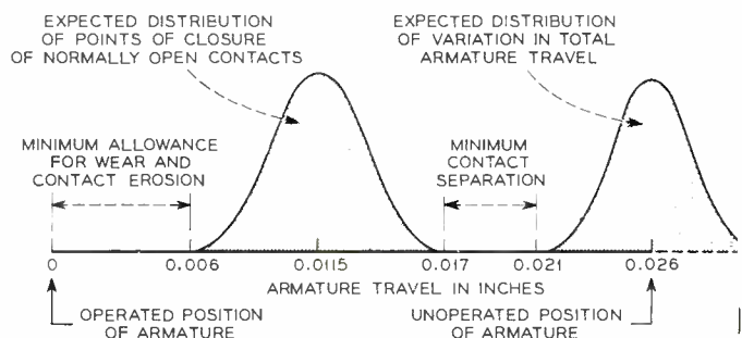
Fig. 2 — Expected variations in contact closure point increase the total armature travel by a like amount.
