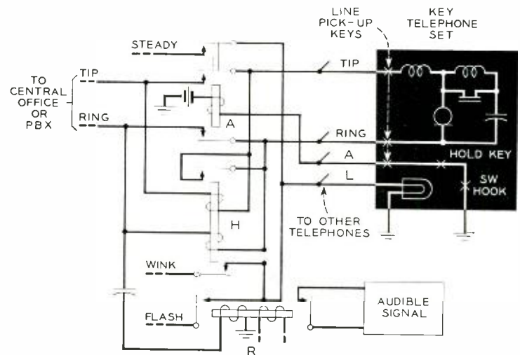
Fig. 2 — Simplified diagram of 1A1 central office or PBX line circuit used in the key telephone system.
