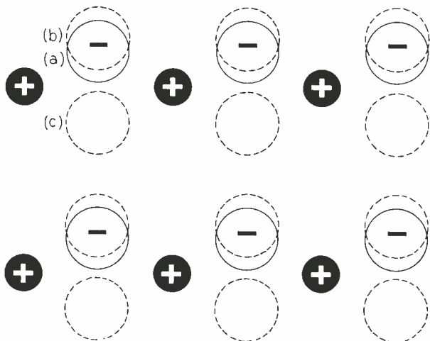
Fig. 3 — Even when no voltage is applied, the center of gravity of the negative charges is displaced from that of the positive charges in a ferroelectric crystal. (a). When you apply a voltage producing the field E in one direction, (b), you increase that displacement, and when you remove that voltage, the displacement returns to its original value, (a). A large enough voltage in the other direction, however, “switches” the crystal, and when you remove that voltage, the displacement (c) looks like (a) upside down. Thus the crystal is what apparatus engineers term a “bi-stable device.”
