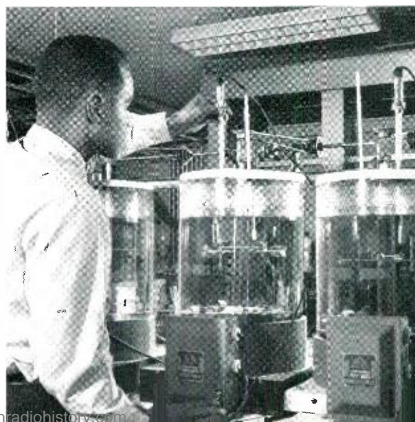
Fig. 5 — C. E. Miller uses the reciprocating rotary crystallizer, developed by the author to grow ADP crystals during World War II, to grow crystals of G.A.S.H. from a water solution.
