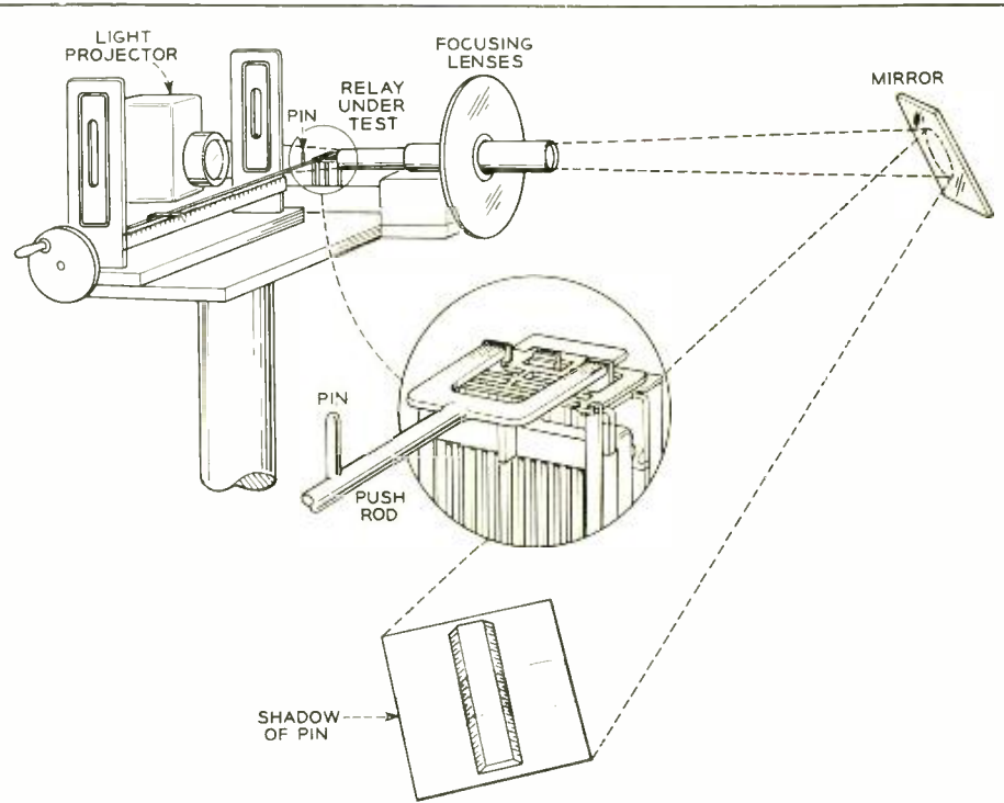
Fig. 3 — Diagram illustrating operation of relay load-displacement tester shown in Fig. 1.
