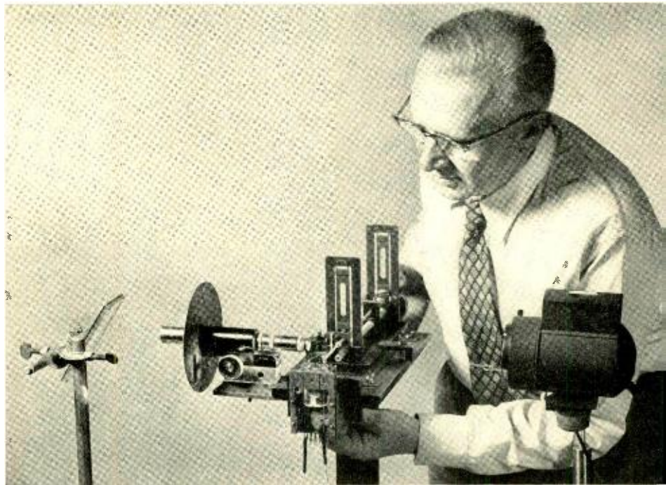
Fig. 1 — J. L. Agterberg applies calibrated tension to relay springs as an optical system registers the resulting displacements.
