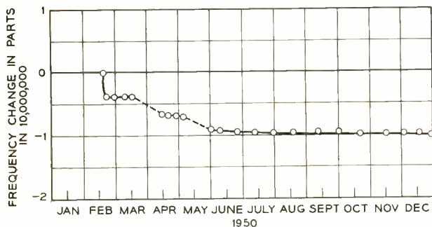
Fig. 4—Graph indicating the frequency aging characteristics of a 10-mc crystal unit enclosed in a 60 degree oven and tested in the indicated circuit.
