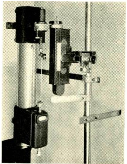
Fig. 4 - Calibration of the new extensometer.
