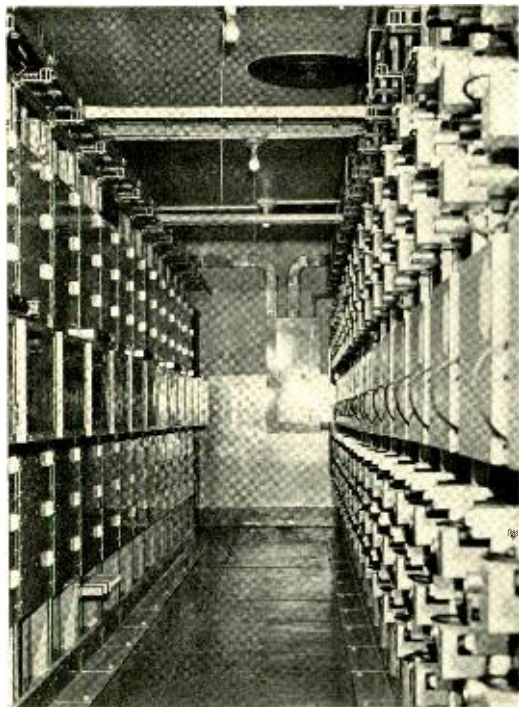
A view of the bays containing the thirty-four record-reproduce machines, amplifiers, and associated equipment required by the system.
