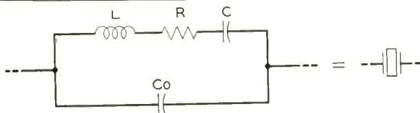
Fig. 6—Electric circuit with characteristics equivalent to those of a vibrating crystal.
