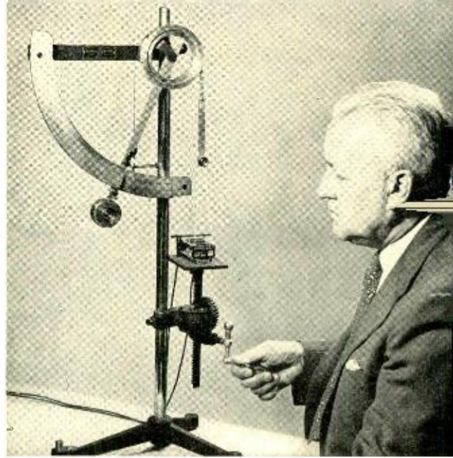
Fig. 1 — R. Calame operating relay pull tester.
