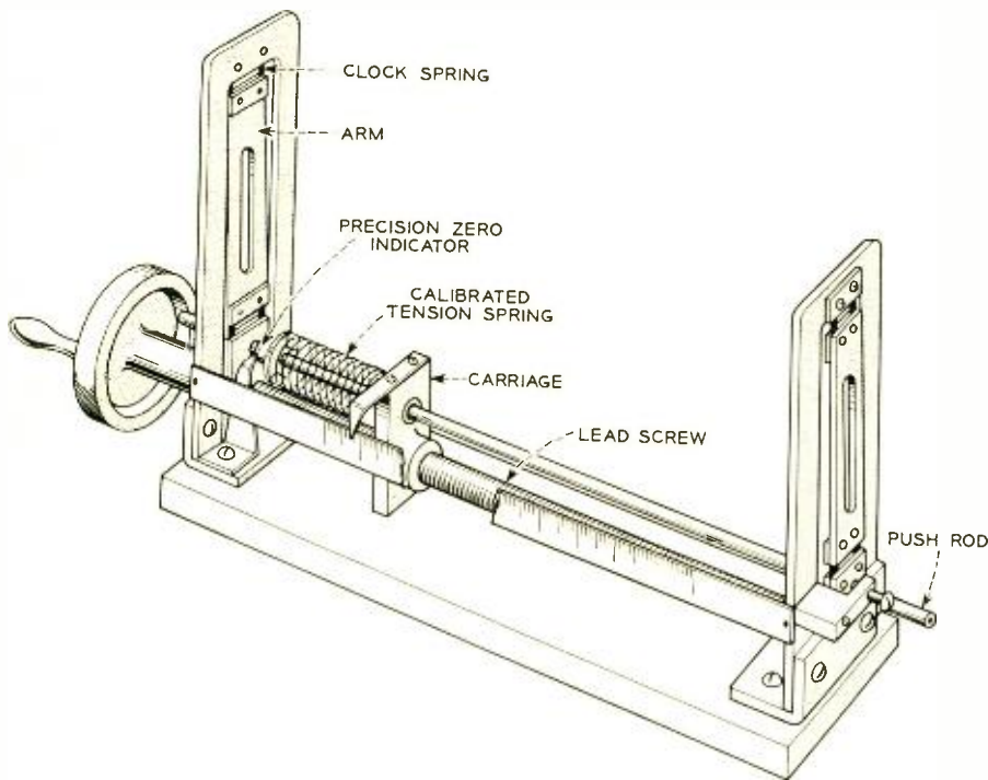
Fig. 2 — Frictionless spring balance.
