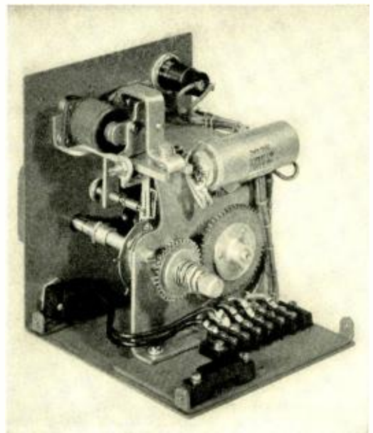
Fig. 2 — The synchronous drive motor drives the right-hand gear from behind the mounting bracket.
