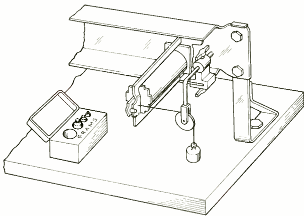
Fig. 4 - Weight method for measuring relay pull.
