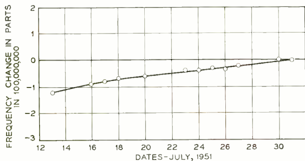
Fig. 5—Frequency aging characteristics of a 5-mc crystal unit during the first three weeks of its life.
