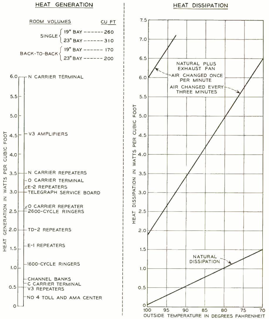
Fig. 4 — Heat generation and dissipation in Type-N terminal offices.
