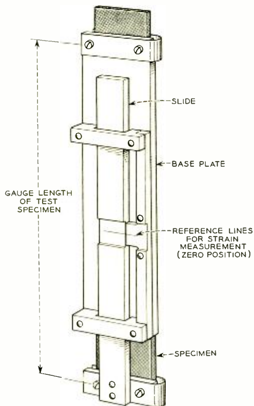
Fig. 1 - Extensometer formerly used for creep studies. The fine line shown across the center section of both the base plate and the slide is shown in the zero (unstressed) position. As the test specimen lengthens under the applied stress, the amount of separation between the lines gives a measure of the strain.
