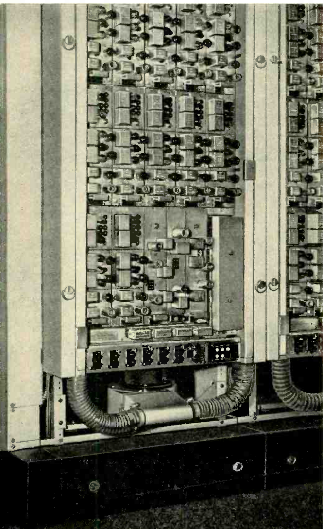
Fig. 3—Each relay rack bay of type-N carrier equipment is provided with a small blower. Air from this blower is conducted through the rectangular ducts at the sides of the bay and discharged near where the electron tubes are concentrated.
