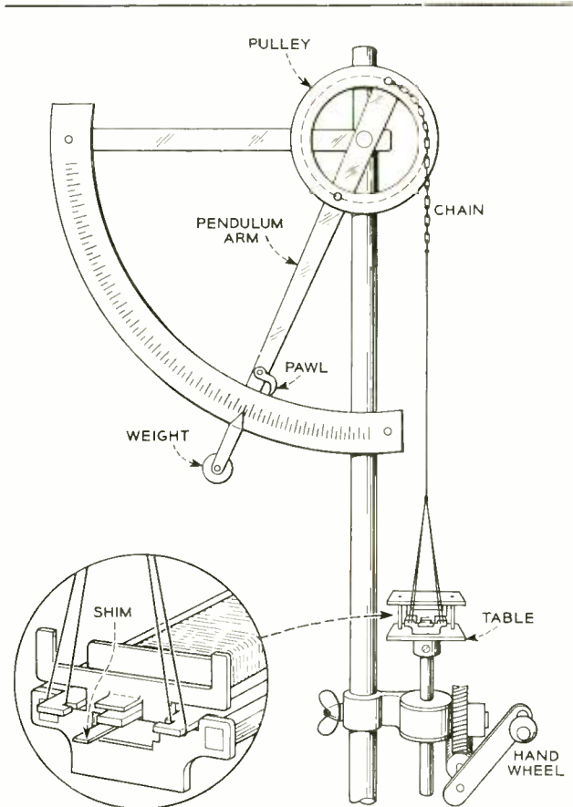
Fig. 5 - Pendulum method for measuring relay pull.
