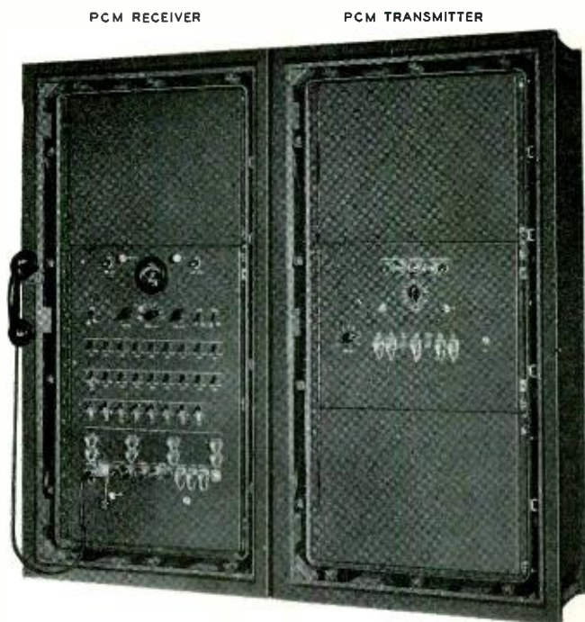
Terminal apparatus for an eight-channel PCM system using a five-pulse binary code
