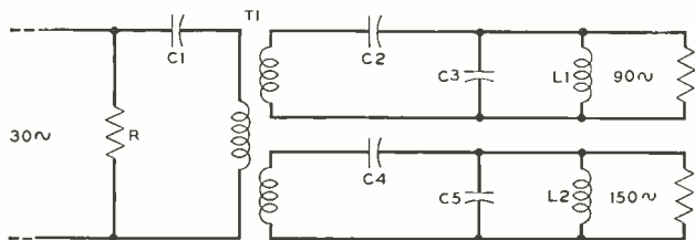
Fig. 4—Frequency generator circuit
