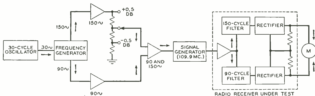
Fig. 2—Block schematic of the circuit designed for testing runway localizer receivers
