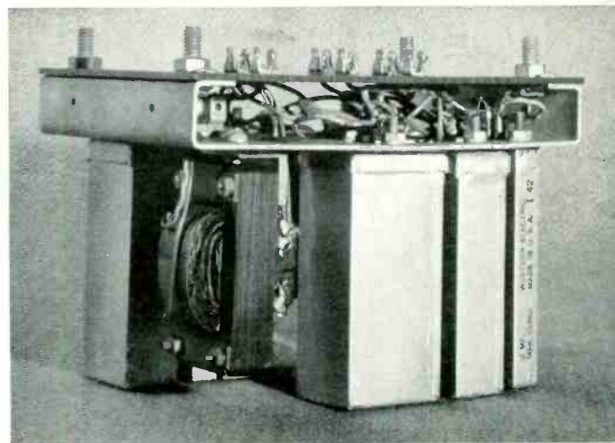
Fig. 3—The coils and condensers forming the frequency generator are mounted on a metal chassis attached to the underside of the cover of the container
