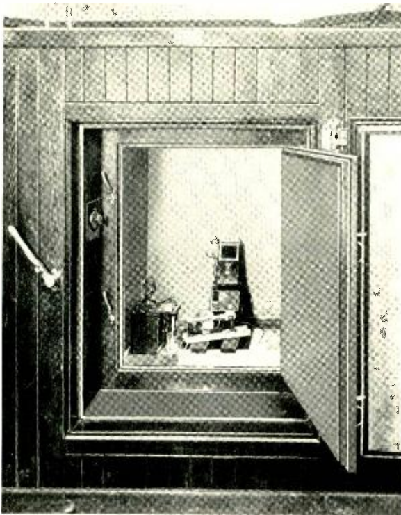
Small air-tight chamber for accurate humidity control
