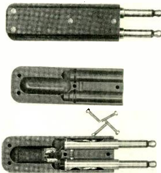
Twin plug with resistance unit, for balancing toll circuits during testing
