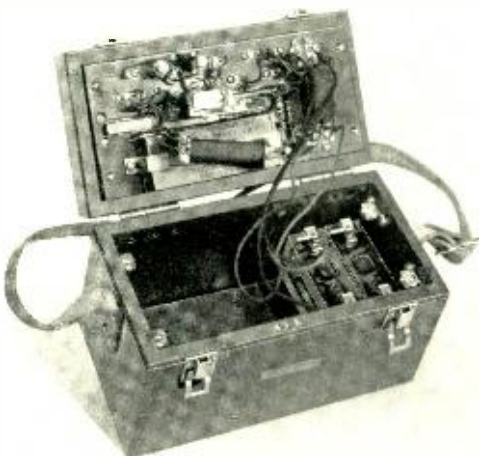
Circuit members assembled on lower side of the panel
