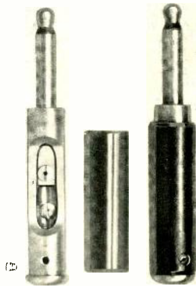
The No. 47 plug, used for test boards, magneto switchboards and private branch exchanges
