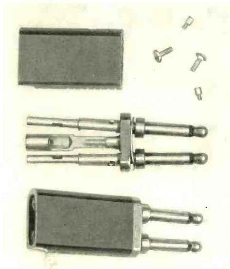
Twin plug used at toll test boards
