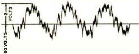
Fig. 3. Voltage wave of a typical commercial-type generator
