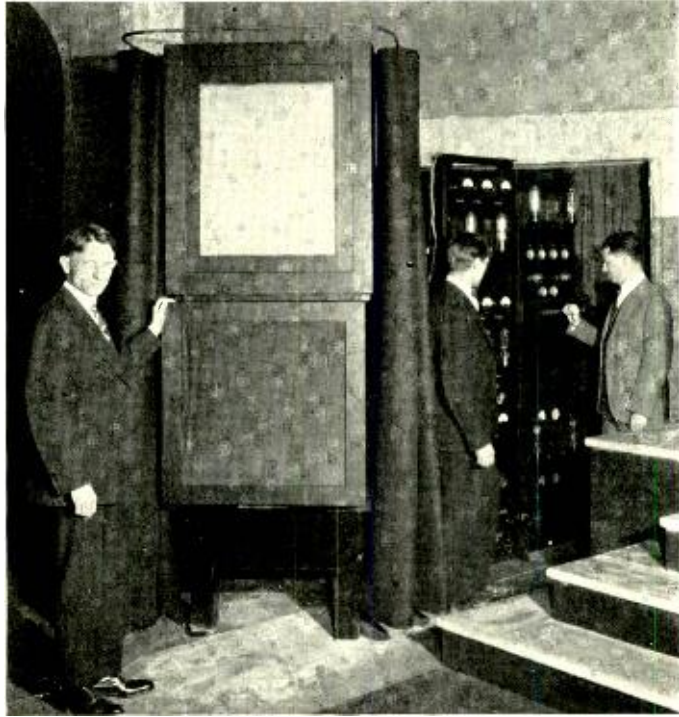
One form of receiving apparatus for television; the distant scene is made visible to the audience on the glass screen in the center of the picture. Dr. Frank Gray, who is largely responsible for that method of receiving, stands at the left, his hand resting on a lower screen behind which is the loud-speaking telephone. On the right, W. S. Bishop and E. Peterson manipulate the controls of the amplifier and other associated equipment
