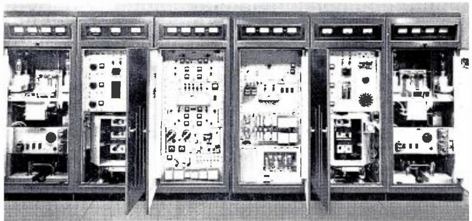
THE TRANSMITTER that is making UHF history in Easton and Columbia—the Du Mont 5 KW UHF television transmitter is reported to be breaking all records for dependable, strong coverage. The transmitter represents a new concept in UHF design as a result of the use of the high-gain Eimac klystron final amplifier. Low operating costs are noted by station engineers who have welcomed the trouble-shooting system built in Du Mont transmitters as well as the convenient dolly-mounted final Eimac klystron. The unit is housed in six cabinets, shown here with doors open. All adjustments and maintenance points are readily accessible.
