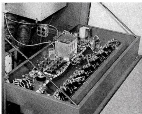
Easy Access Drop-Down Meter and Control Panel
