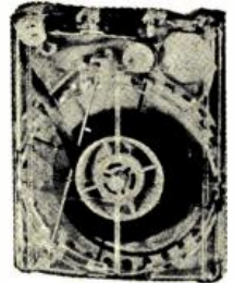
STANDARD FIDELIPAC CARTRIDGE
