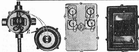
Box with terminals, cable support, and receptacle in cover. Box with factory installed screw cap receptacles. Box with special terminals and cable support.
