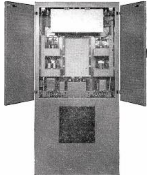
(Left) Collins 300J 250/100 watt AM broadcast transmitter.
