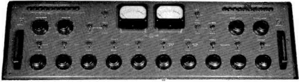
Collins 212A speech input console, above. Facilities are provided for auditioning or rehearsing, cueing and broadcasting simultaneously from any combination of two studios, an announce booth, a control room microphone, two turntables, and any two of nine remote lines. Two program amplifiers are included, making possible the feeding of two independent programs at
