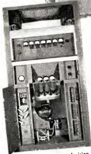
One of the Du Mont television transmitter units—5 KW Visual Amplifier, with three built-in cathode-ray indicators.
