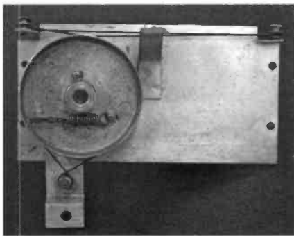
This is the dial mechanism from the back after cleaning and re-stringing.
