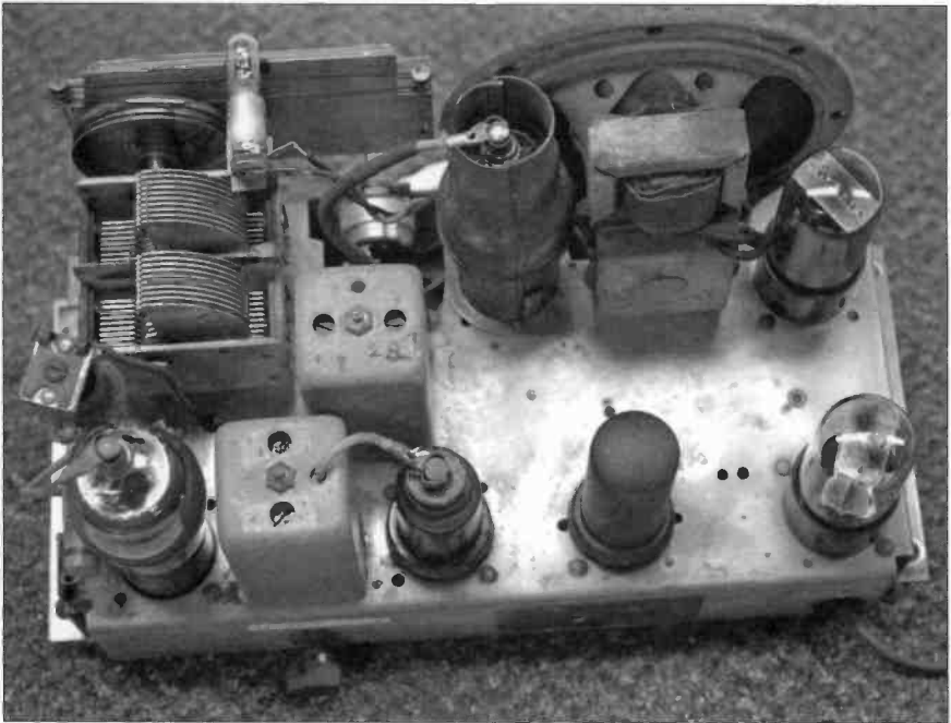
Here's the completed chassis cleaned up and ready for alignment.
