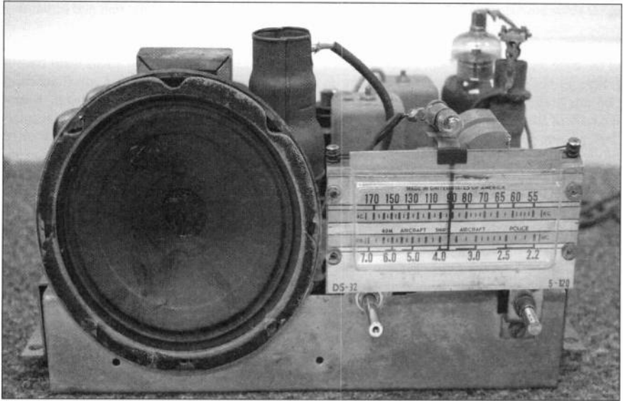
A nice clean chassis ready to put into the cabinet.
