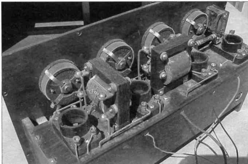
Rear view of the Timmerman chassis showing the assembly of purchased parts from other manufacturers.
