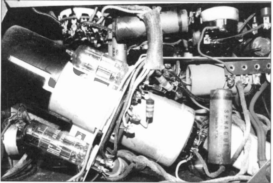
Inside view from left side of scope with cover off
