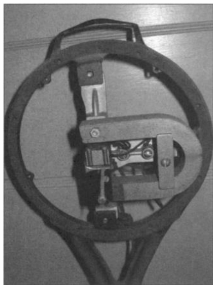
Driver and base with cone removed
