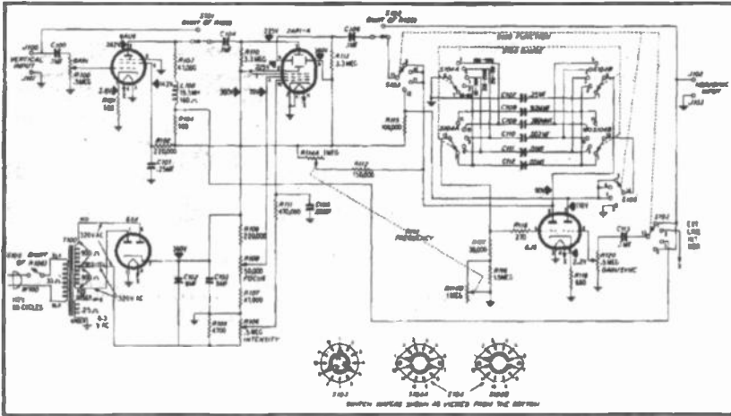
Figure 25. Complete Schematic
