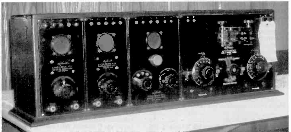
The DeForest Interpanel set with coils, but without tubes, in very good condition, sold for $1,500.
