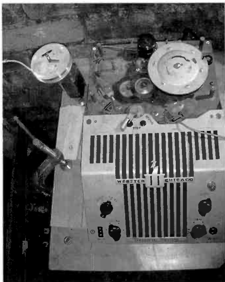
Figure 3. The Webster-Chicago Model 180 used by the author to recover his grandfather's old recordings.
