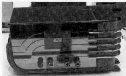
From the contest, a nice Sparton Model 557 "Sled" blue-mirrored radio.
