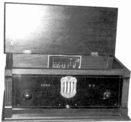
Figure 1. The Long Model B5, ca. 1926, has NA-ALD brand dials, five Type 01-A tubes, three binocular coils, and a thumbwheel dial.
