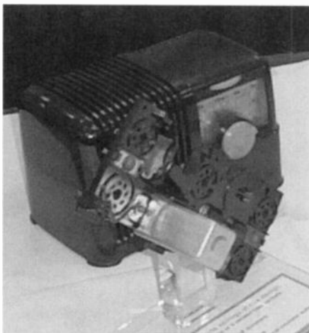
This contest display shows a Zenith table radio utilizing a one-piece Bakelite chassis with mold-in tube sockets.
