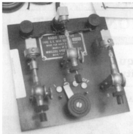
A rare 1916 Wireless Specialty Apparatus Co. SE-183A triple crystal detector in the equipment display.
