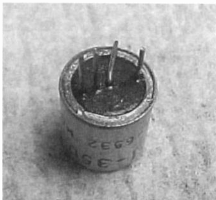
Figure 1. A bottom view of one of the transistors used in the Zenith Royal 3000. From left to right, the leads are emitter, base, case ground and collector. Note that the case ground pin has been bent over so that it will not make contact with the socket.
