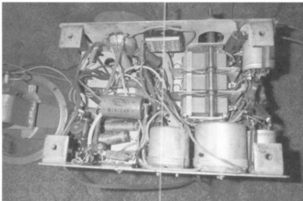
Figure 4. The bottom view of the chassis shows the crammed in components.
