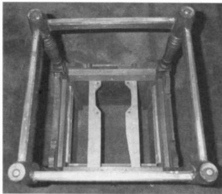
Figure 5. The metal strips located under the cabinet's leg stretchers serve as the radio's antenna.
