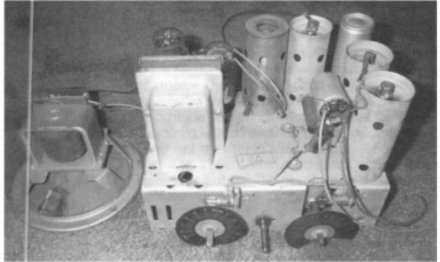
Figure 3. A top view of the GE K-60 chassis.
