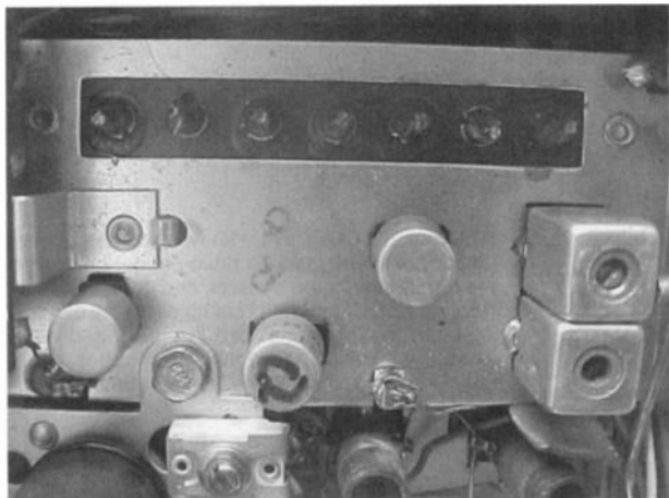
Figure 2. This view of the radio's AM tuner chassis shows the three transistors in their sockets.
