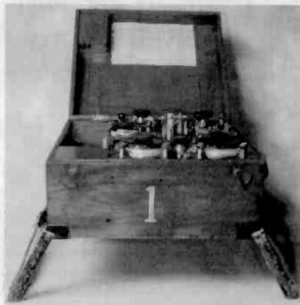
Figure 1. A Mark III Short-Wave Tuner in its case with the support legs in the extended position.
