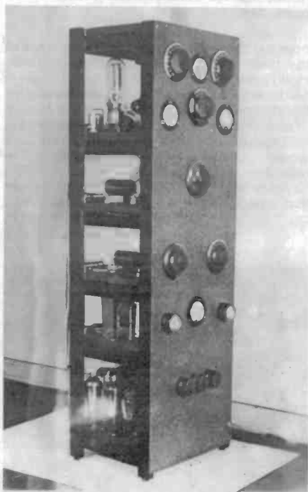
Figure 6. A superb example of an early home-brew transmitter.
