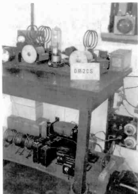
Figure 2. A closeup of the transmitter used at the Guam "lash up." The coils are wound from copper tubing. The 20-meter coils are in place. The 40-meter coils are on the bottom shelf next to the power supply.
