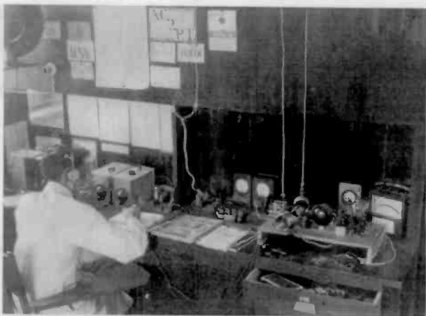
Figure 5. Also from the Far East, a Ham station with home-brew equipment. Note the plug-in coils and the callbook on the operator's table.
