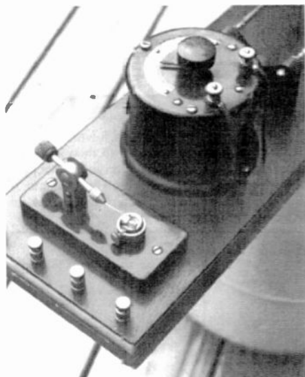
Figure 3. This view shows the Murdock tuning condenser and the crystal detector at the far end of the board.
