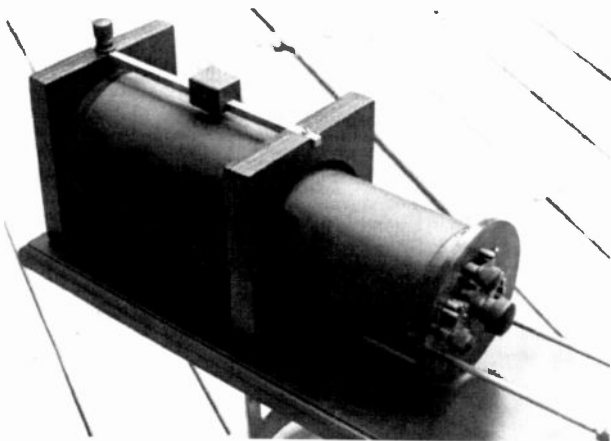
Figure 2. The Arlington-type loose coupler mounted at the end of the board. The coils are wound with fine, black, cotton-covered wire.
