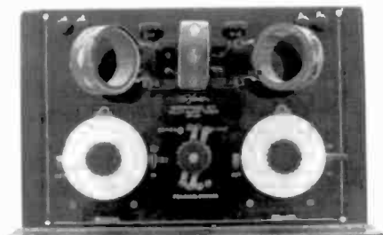
DEFOREST MT-200 – This 1921 component has no tubes and is a Multiwave Tuner only. It tunes from 150 to 25,000 meters. This is the tuner section of the DeForest MR-6 Inter-panel 3-tube receiver. (Ross Mason – Mascot City, IA)
