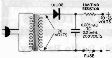
Figure 3. A basic schematic diagram for the 72-volt battery charger. We have added the limiting resistor to Pinelli's design. See the sidebar for additional information
