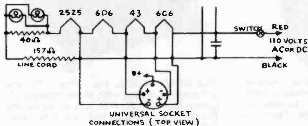
Figure 4. A partial schematic diagram of the Warwick models shows the filament to socket connections.
