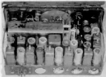
The SCR-300-A with cover removed showing interior components.
