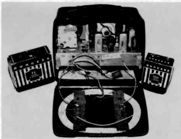
Figure 4. The Emerson Model 560A with rear cover open and batteries removed. On the right side is the Burgess No. XX45 67½-volt B battery converted to a 72-volt rechargeable. On the left side is the Burgess No. F3 4½-volt A battery converted to 4½-volt rechargeable.
