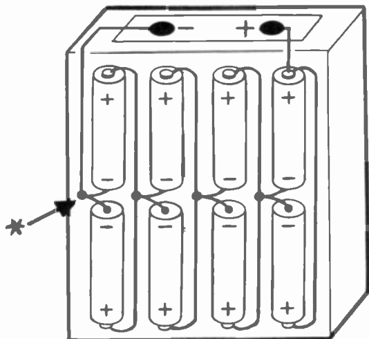
Figure 2. Pictorial diagram of the battery arrangement and wiring for the 4.8-volt A battery. It uses eight 1.2-volt nickel-cadmium, rechargeable C-size batteries wired in series-parallel. The negative ends of the batteries are soldered together using "Solder-Wick." A 0-30-volt, 3-amp regulated power supply is used to charge the A battery.
