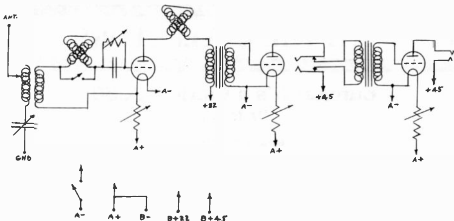
Figure 3. This schematic diagram depicts the circuitry of this 3-tube radio. The regeneration detector is followed by 2 stages of audio amplification.
