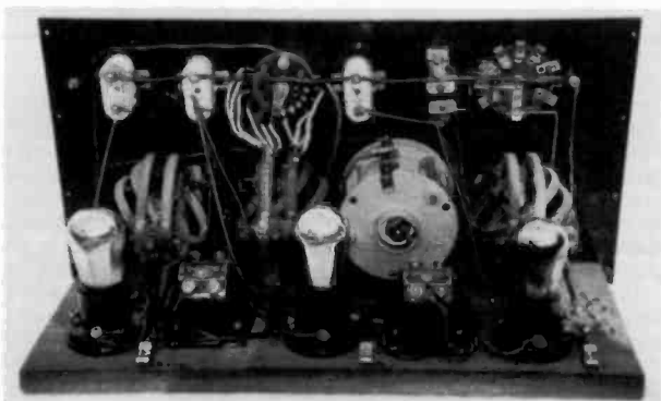
Figure 2. A rear view reveals the neat construction and layout, as well as the author's fine restoration.
