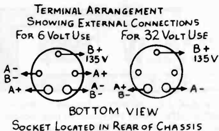
Figure 3. This adapter plug and socket hookup for the Howard Model AA-25 is typical of those found in my search.
