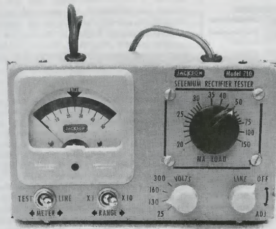
Figure 4. The Jackson Model 710 selenium rectifier tester. Note the meter's "Bad-Good" scale and AC line voltage setting.
