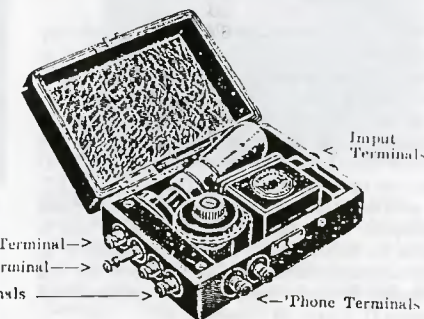
Figure 6. The Sparta one-valve amplifier was built in a case to match the crystal receiver.
