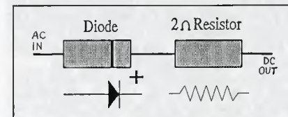
Figure 2. The equivalent circuit of a selenium rectifier.
