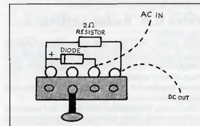
Figure 3. Terminal strip mounting of the silicon diode and resistor.
