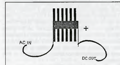
Figure 1. Wiring diagram for a selenium rectifier.
