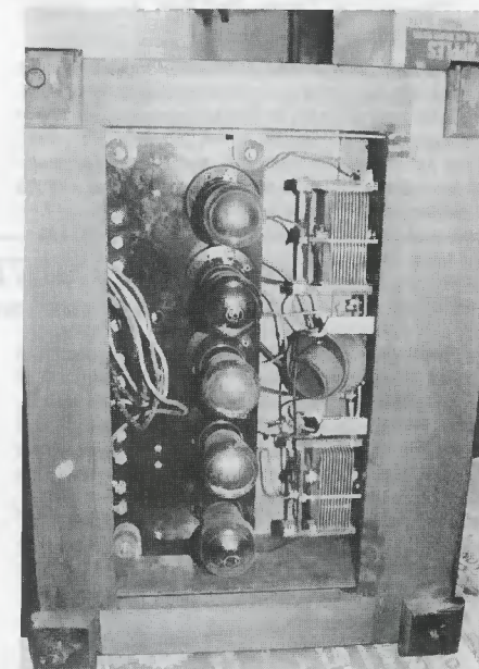
Figure 4. An underside view of the Delano Sheraton shows the radio's tubes and chassis components.
