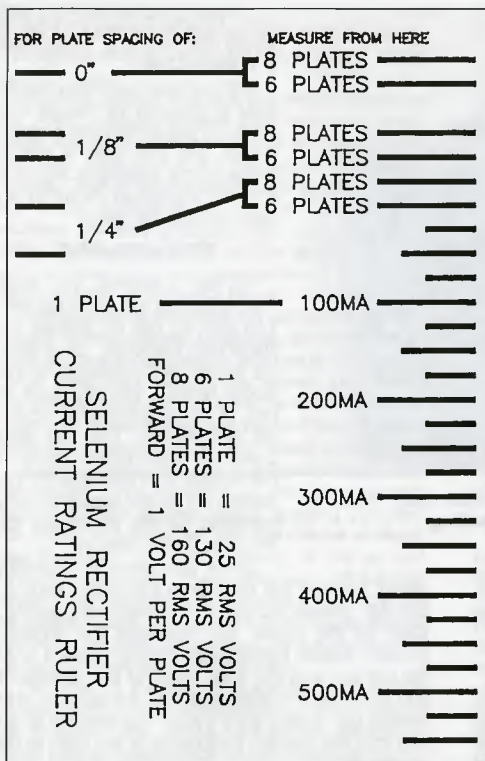
Figure 5. A handy scale for estimating the current rating of a selenium rectifier.
