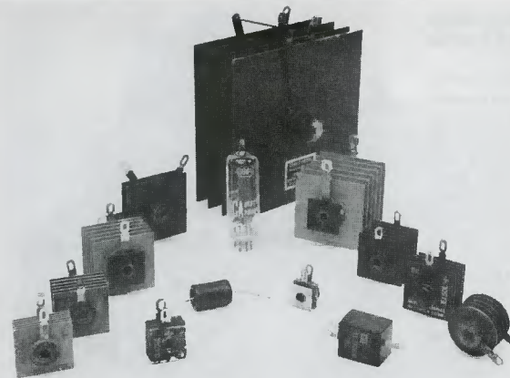
Figure 1 Some examples of selenium rectifiers compared in size to a Type 35W4 vacuum tube rectifier.
