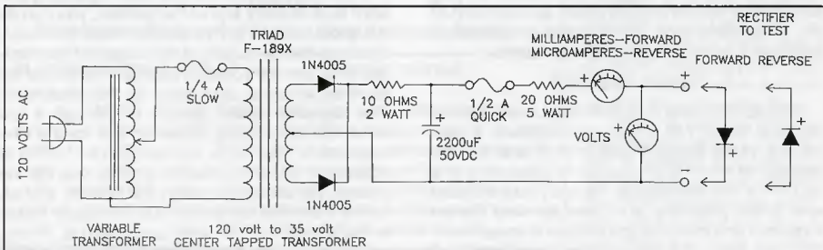
Figure 6. A schematic diagram of a selenium rectifier tester that you can build.
