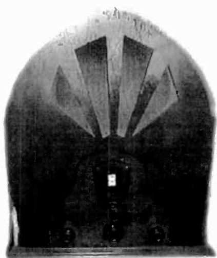
Figure 1. Front view of Scott McCleskey's Automatic Tom Thumb.
