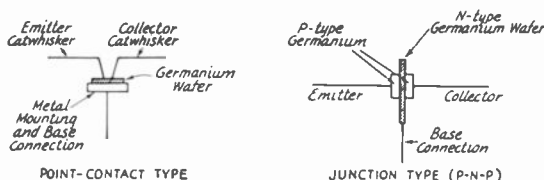
Figure 1. A simplified illustration of the construction of point-contact and junction-type transistors. (From "The Radio Amateur's Handbook" of the American Radio Relay League, 1956, p. 79.)
