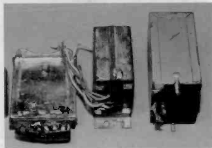
Figure 11. Examples of multisection capacitor blocks housed in metal cans.
