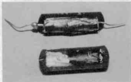
Figure 9. An exploded view of a AC line bypass capacitor that was subjected to excessive voltage.
