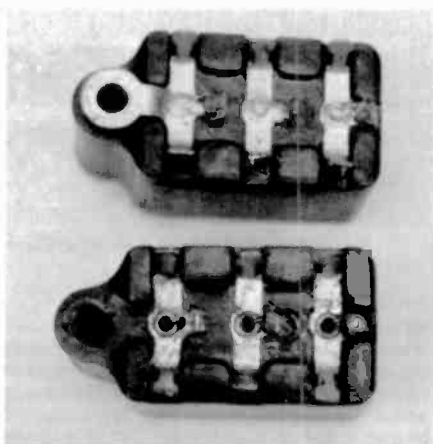
Figure 6. Two examples of the Philco Bakelite block capacitor.
