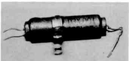
Figure 4. A dual-section tubular capacitor that performs both coupling and bypass functions.
