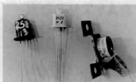
Figure 9. Unusual early junction transistors. Left to right: an experimental GE tetrode or 4-lead device, ca. mid-1950s; a Western Electric 3N22, a production tetrode, ca. 1958; and a Transistor Products power transistor, ca. mid-1950s.
