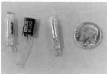
Figure 3. Left: Front of the case of a Sonotone 1010 hearing aid, introduced in 1953. Above: 2 subminiature tubes, and 1 low-noise Raytheon CK718 transistor, shown next to a dime for size comparison. Hearing aids represented the first successful commercial use of transistors.
