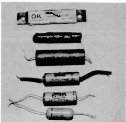
Figure 5. Some typical tubular paper-dielectric capacitors spanning the period from the 1920s to the 1950s.
