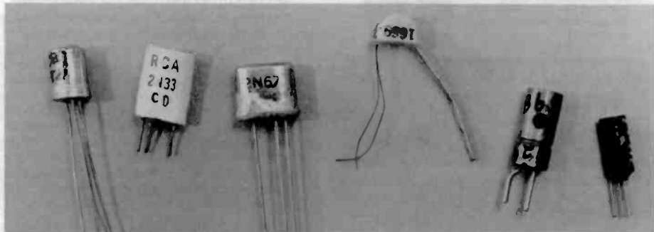
Figure 8: These are somewhat rare point contact transistor types. From left to right: a CBS Hytron, CHY PT-2A of 1954; an RCA 2N33 of 1953; a Western Electric 2N67 of 1954; a Western Electric 1689 of 1953; a Western Electric A1729X; and a General Electric G11. Note the evidence of a small hole in the case of each of the last two units. This hole allowed for adjustment of the fine point contact wires during manufacturing.
