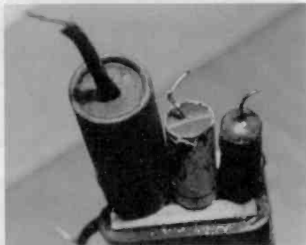
Figure 10. Examples of paper capacitor construction.
