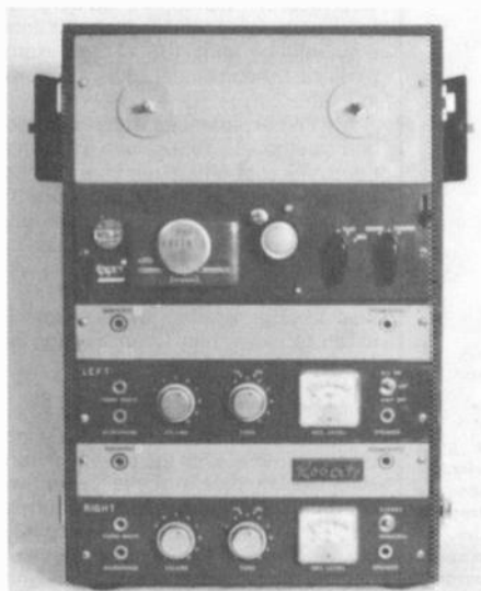
Figure 5. The dual-channel Roberts Model 990, ca. 1961-1962, is an AC-operated, tube-type tape recorder, using 7" reels and running at 15, 7½, and 3¼ ips.
