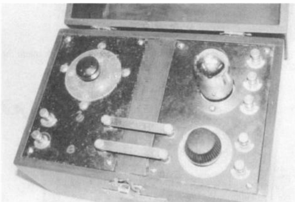
Figure 10. The two panels of the Splendid Jr. Note that the dial crank, as well as the tap switch, used in the Sr. are not used in the Jr. version.
