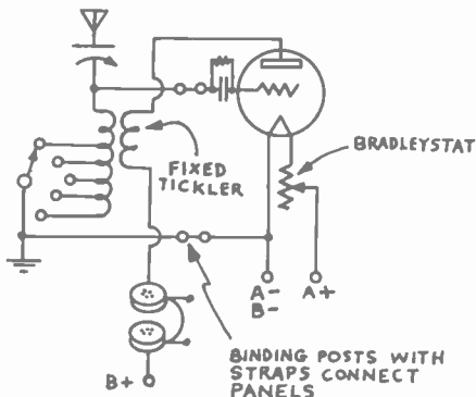
Figure 7. Schematic diagram of the Splendid Sr. regenerative circuit.
