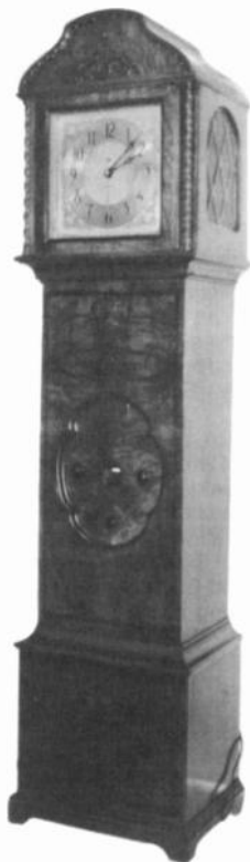
GILFILLAN GRANDFATHER CLOCK RADIO MODEL UNKNOWN – This unusual radio, circa mid-1930s, is only 4' 10" tall. Built on an even more unusual, large aluminum chassis, the radio uses the following tube types: (2) 47, (1) 80, (2) 35, (2) 27. It was designed so that the two Type 47 tubes and the Type 80 are mounted vertically, and the rest of the components are mounted horizontally. A chassis tag reads, "Manufactured by Gilfillan Brothers." ( Jerry DeWitt – Simi Valley, CA )
