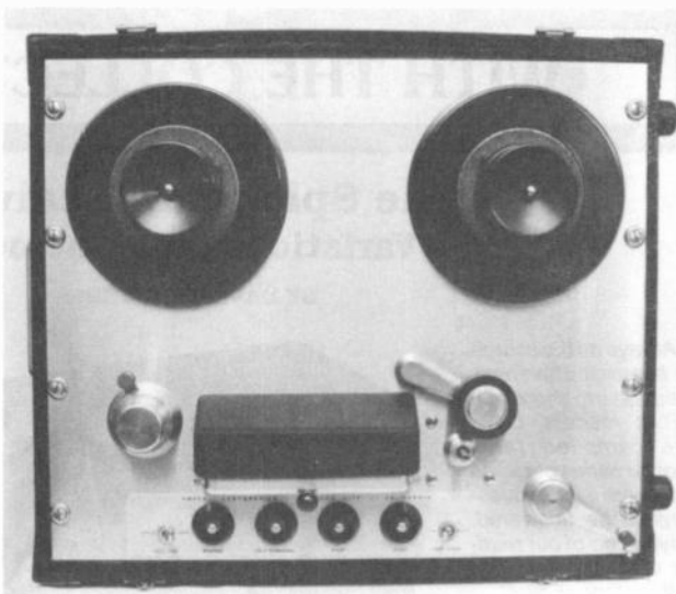
Figure 7A. The tape transport of the Ampex Model 350 series, ca. 1953-mid 1960s. A studio quality, 3-motor, 3-head transport, it operated at 15 and 7½ ips or 7½ and 3¾ ips and accepted reels up to 10½".
