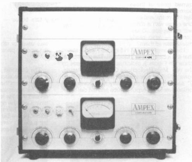
Figure 7B. The dual-channel, tube-type electronics of the Ampex Model 350 series.
