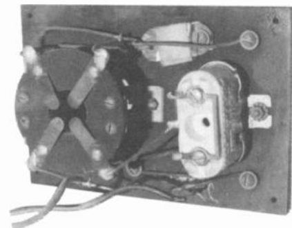
Figure 6. An underpanel view of the right-hand detector panel.
