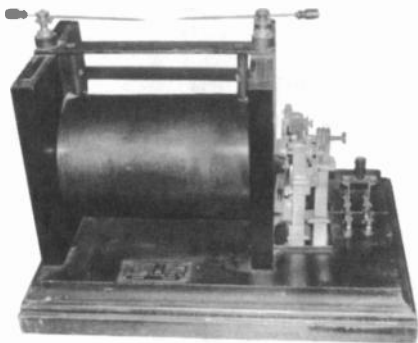
THORDARSON MODEL 8508.6 – This unique spark coil mounted on its original board measures 18" x 12½" x 14". The coil is 8½" in diameter. ( Steve Lange – Milwaukee, WI )
