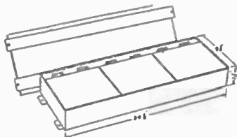
LONG "D" BATTERY CONTAINER No. 21932 FOR USE WITH MODEL 81-B OR 81-C.
