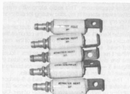
Figure 3. The Atwater Kent spark plug suppressors.
