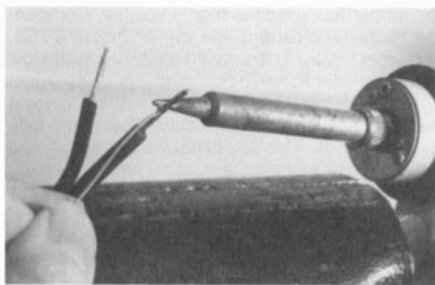
Figure 8. Tinning a line cord wire before soldering it to the terminal gives better results than attempting to solder the wire without tinning.
