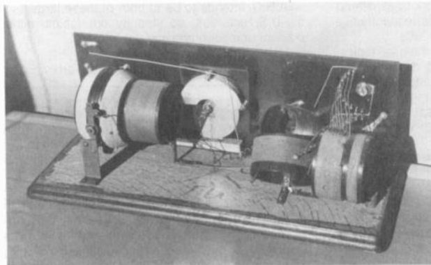
Figure 2. The RA-10 interior showing the unique mounting of its components.
