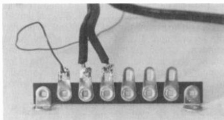
Figure 5. Three examples of poorly soldered joints: Left and center: There is solder on the terminals, but the wire did not tin because of insufficient cleaning. Note that the solder has not flowed onto the wire. Right: There was insufficient heat to make the solder flow on smoothly. Note the dabbed-on, spiked look at the top of the joint.
