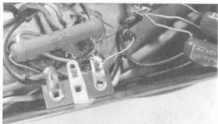
Figure 10. This is a typical terminal lug. Note that the right-hand lug has wires crimped on it and is ready to solder.
