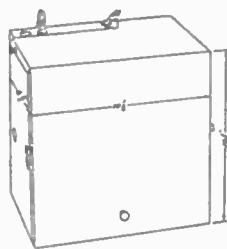
MODEL 81-B CHASSIS AND "C" BATTERY CONTAINER No. 21929. (For dash mounting.)
