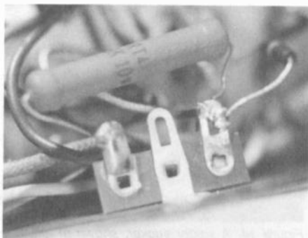
Figure 13. This is a good solder joint. Note the smooth appearance of the solder as it completely surrounds the wire and terminal.
