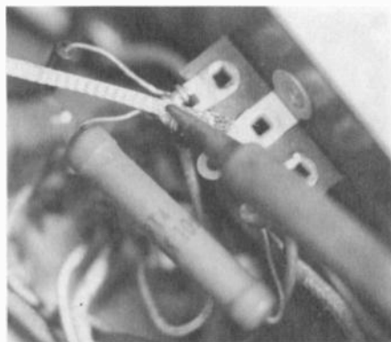
Figure 15. When you remove solder with a wick, the wick should lie across the joint where it can contact the bulk of the solder.
