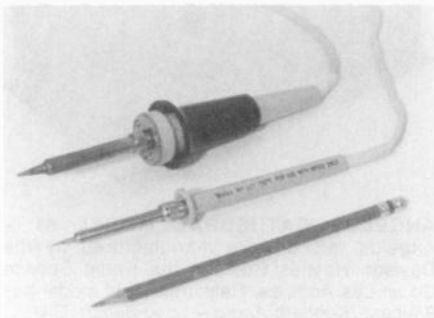
Figure 1. A standard size Weller iron and a miniature Weller iron for small work, shown with a pencil for size comparison.
