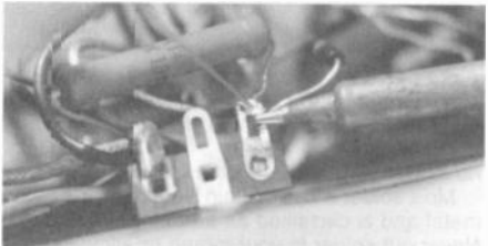
Figure 11. The right-hand lug is now ready to solder. Note that a small amount of solder is applied to the soldering iron tip and the joint, just at the point where they touch.
