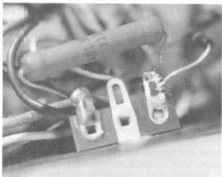
Figure 12. The top lug has been poorly soldered with insufficient solder to cover all the wires.
