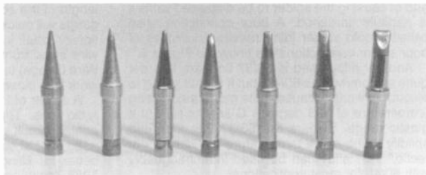
Figure 4. Commonly used soldering tips are these Weller types, from left to right: PTP 0.031" conical, PTH 0.031" screwdriver, PTA 0.063" screwdriver, PTAA 0.063" single flat, PTB 0.094" screwdriver, PTC 0.1125".
