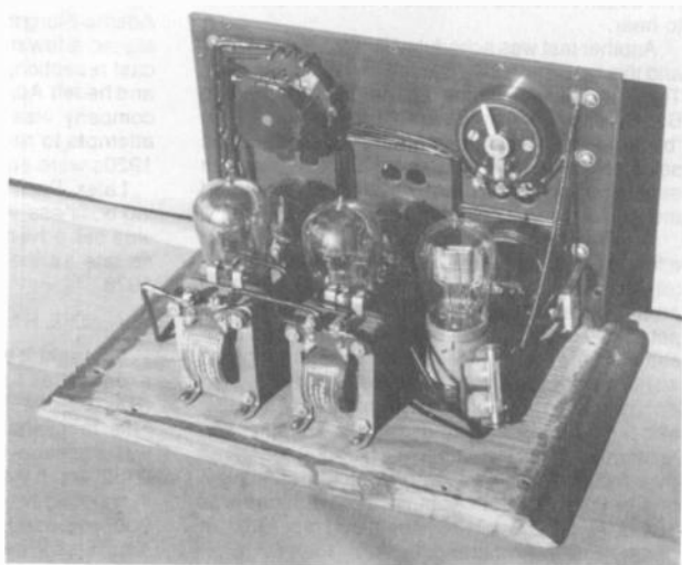
Figure 4. The DA-2 interior. Note the nonoriginal gridleak and by-pass condensers.
