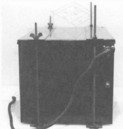
Figure 2. The enclosure for the chassis and battery box. The shielded antenna cable is shown in the upper-right-hand corner. Directly below is the receptacle for the mechanical tuning cable. Note the top and bottom mounting brackets and mounting bolts for under-the-floor installation.
