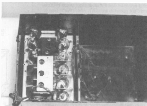
Figure 5. Interior view of the chassis and battery box. The multiwire cable is for connecting all B and C batteries. Note the angle bracket in the middle rear of the chassis with receptacles. A 2-plug cable for the speaker brings all connections for output transformer, speaker and volume control through a cutout in the top edge of the box.
