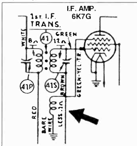
Figure 1. The mysterious third winding on the secondary of the first IF transformer. This schematic is from Rider's Volume VII, page 7-73.
