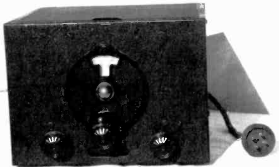
Figure 2. The National SW-3, a 3-tube regenerative receiver, has a dial straight out of the 1920s.
