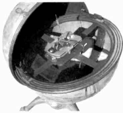
Figure 3. The Symphonic's paper cone is removed to show how the permanent magnet driver is mounted. By looking into the bottom, you can see how the grille cloth covers each of the lower openings.
