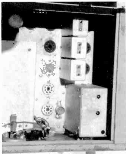
Figure 6. The two miniature tube sockets on this NC-173 chassis were "improvements" which smoked the power transformer.
