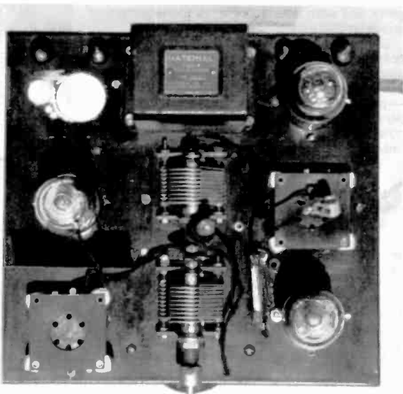
Figure 4. The originality of this National SW-3 chassis has been destroyed by the addition of several holes in the upper left corner.
