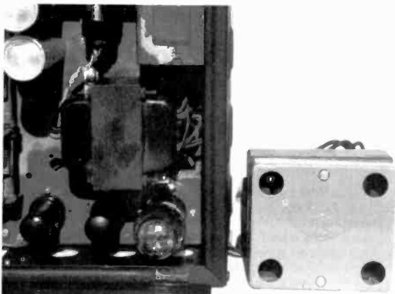
Figure 7. A National NC-100 with a replacement transformer (left) and an original power transformer (right).
