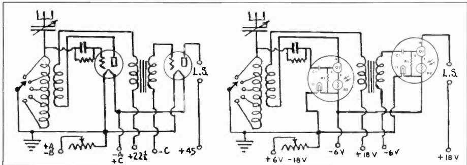
Figure 5. On the left, the schematic diagram for a Crosley Model 51 using Type 01-A vacuum tubes. The schematic diagram on the right shows the radio with tube substitutes in use.
