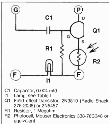
Figure 1. The schematic and parts list for the solid-state tube substitute.
