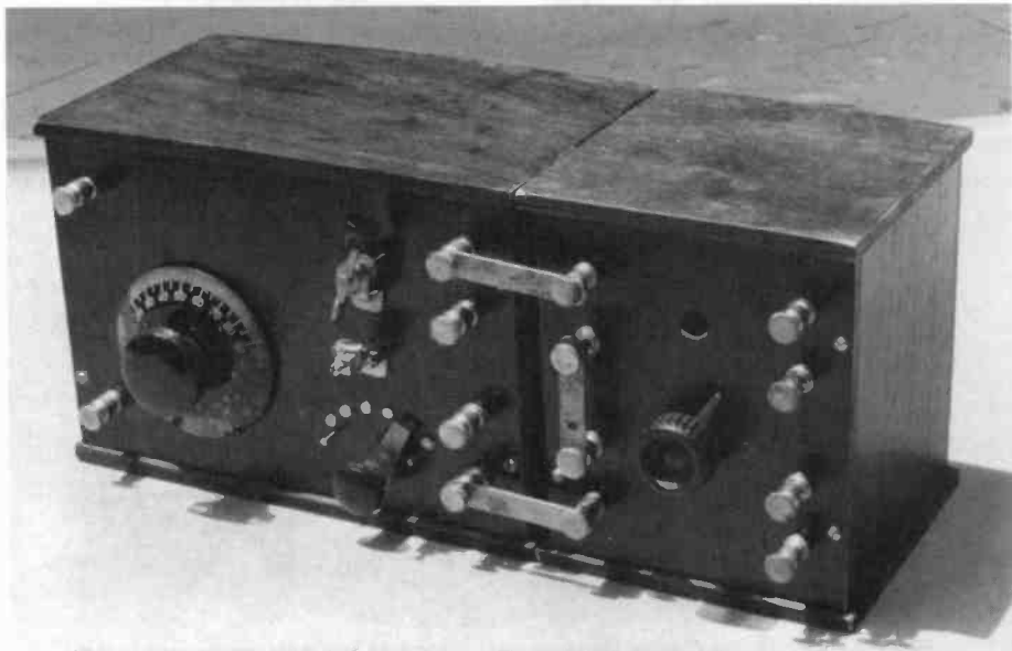
Figure 6. The Harko set connected to the Crosley Audion detector for tube detection.
