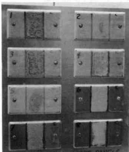
Figure 1. This test panel contains the zinc-plated junction box covers on which cleaning agents 1-8 in Table I were applied.
