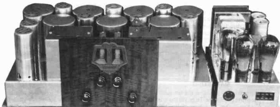
Figure 2. The Scott Allwave Superheterodyne.
