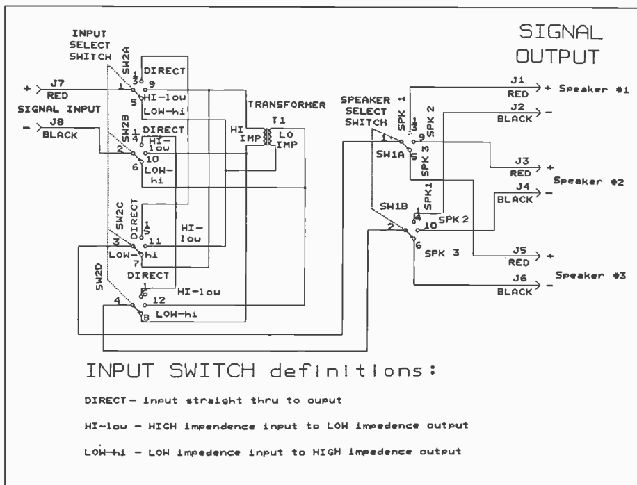
Figure 4. Schematic diagram.
