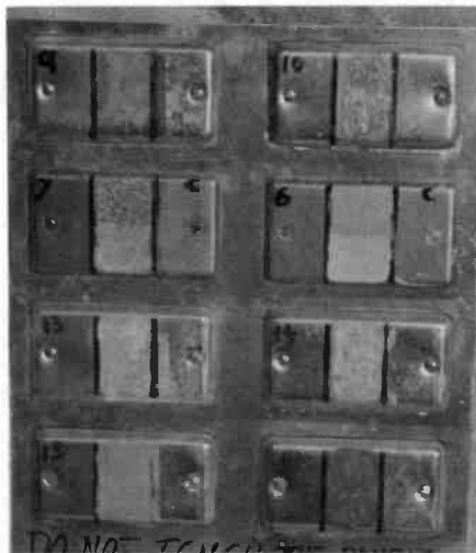
Figure 2. This test panel contains the box covers on which cleaning agents 9-16 in Table I were applied.
