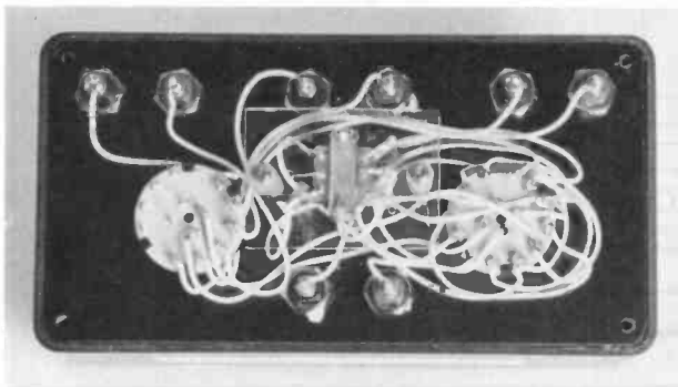
Figure 3. Rear view showing internal wiring.
