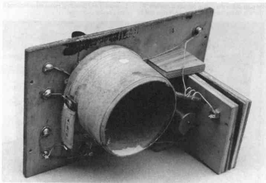
Figure 4. Interior of the Crosley Har-ko crystal set showing its simple, crude construction.
