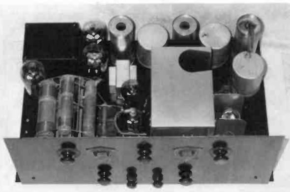
Figure 5. Top view of the Silver-Marshall Model 726SW chassis.
