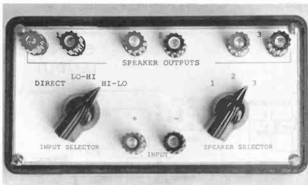
Figure 2. Front panel of the hornbox.
