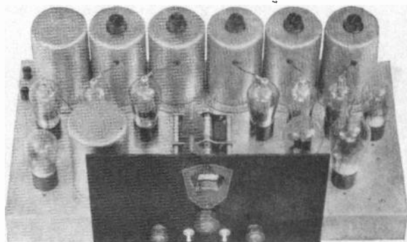
Figure 8. The Lincoln Model 31 from a photo in "Radio News," October 1930.
