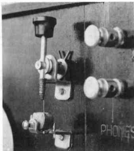
Figure 5. Close-up of the crystal detector used on the Crosley Harko crystal set.
