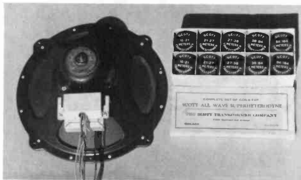
Figure 3. The 11-inch Rola speaker used in the Scott Allwave and a complete set of coils for the shortwave bands.
