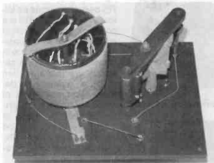
Figure 3. Interior view of the Fellocryst Super, showing a compression-type variable condenser.
