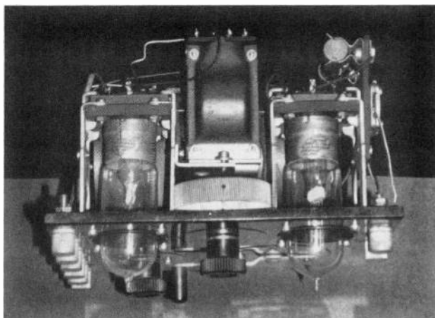
Figure 3. Another view of the Radiola RS chassis showing the two Type WD-11 tubes.
