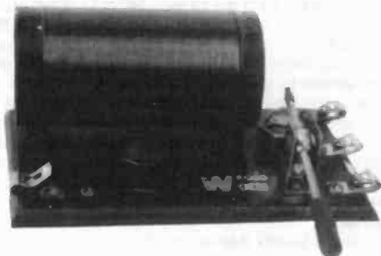
WECCO GEM CRYSTAL SET – This set was made by William E. Cheever, Co., in Providence, Rhode Island. The date of manufacture is unknown. (Frank White – Olathe, KS)
