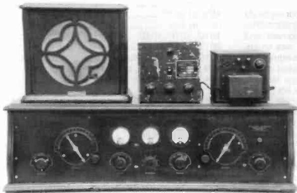
NORDEN-HAUCK ADMIRALTY SHIELDED MODEL SUPER 10 – This 10-tube TRF model is shown with a Norden-Hauck Model N-40-A electrodynamic speaker and a Model 550 B and C eliminator. The A eliminator is a Knapp Model 29. Original documents show the unit was purchased in January 1929. (John Kelly – Ashton, MD)
