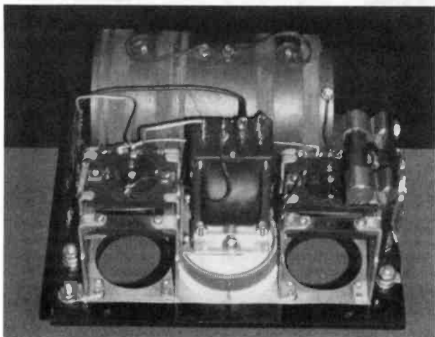
Figure 2. The chassis of the Radiola RS.
