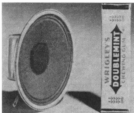
Figure 2. This P275-Y Jensen speaker, 2.75 inches in diameter, was developed for the Regency TR-1. It has a 16-ohm voice coil and weighs less than 2.75 ounces. (Photo from "Radio and Television News," March 1955.)
