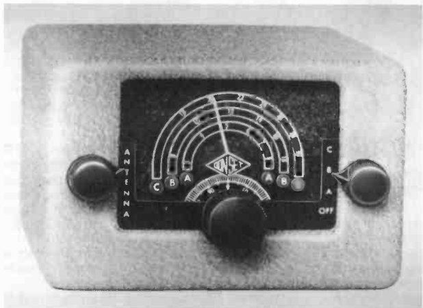
Figure 11. The Gonset 3-band converter, tuning from 3 to 30 MHz.
