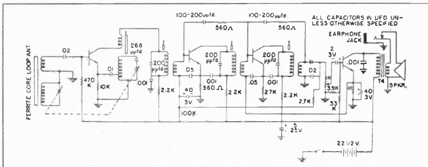
Complete schematic for the Regency Model TR-1.
