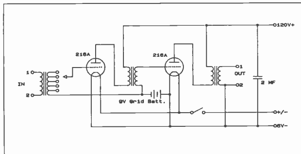
Figure 4. Circuit diagram of the Western Electric amplifier.
