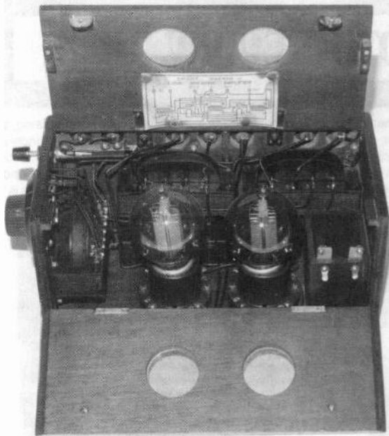
Figure 3. Internal view of the Western Electric amplifier with the top and frontpiece opened showing the two Western Electric Type 216A tubes.
