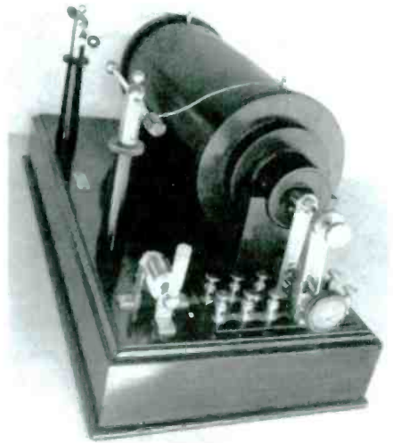
Figure 8. Marconi ten-inch Spark Coil. Similar spark coils were used in the early 1900s as ship-board transmitters and after 1912 as emergency transmitters. A tuning helix and 600-meter loading coil was used with this particular spark coil, made in 1908.
