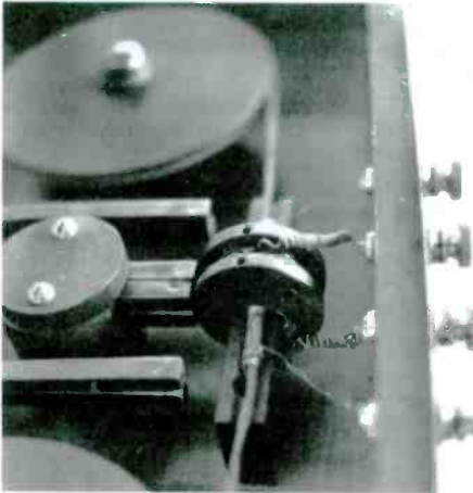
Figure 7. Interior view of the Marconi Magnetic Detector. This design makes use of an endless loop of iron wire running on two clockwork-powered spools. The wire slowly passes through a small glass tube on which are wound two coils. One coil is connected to the antenna or tuner and the other to a headset. Two magnets are mounted close to the coils.
