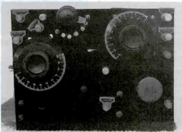
Figure 1. A one-tube homemade set.
