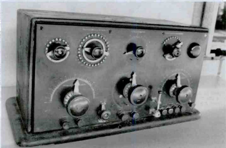
Figure 11. Marconi Model 106 Receiver. From 1912 to 1919, the Marconi Company developed twenty-one receivers, numbered 101-121. The 1915 version of the 106 receiver contained both a crystal and a Carborundum detector. The 106 was built in large quantities for shipboard use in World War I. Later versions, the 106-B and the 106-C, were built by General Electric for RCA.
