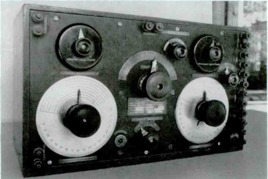
Figure 13. Marconi Type CM294C Shortwave Tuner. This unit was made in 1917 for the U.S. Navy. It was one of four sets used as a standby for transmitting monitoring at the Bolinas, Calif., transmitting station. It is a tuner only and requires an external detector. Its wavelength range is 250-3100 meters.
