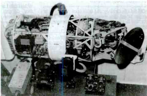
Figure 1. The APS-4 radar system.
