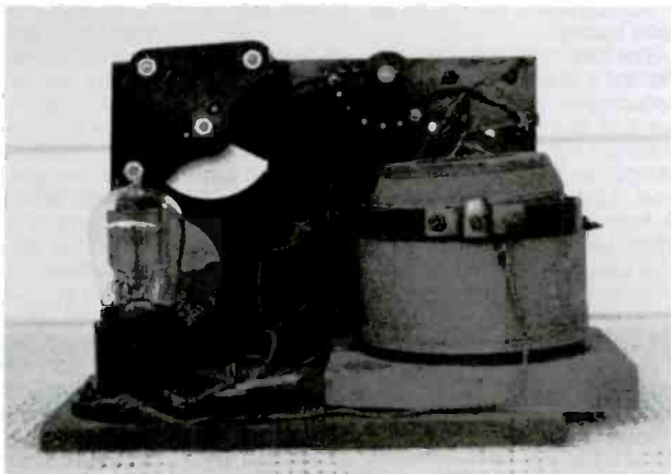
Figure 2. Back view of the one-tube homemade set.
