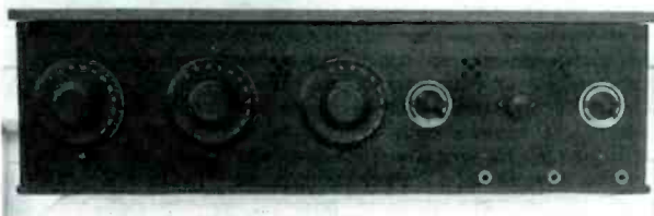
Figure 4. A well-made, home-built, five-tube TRF set.
