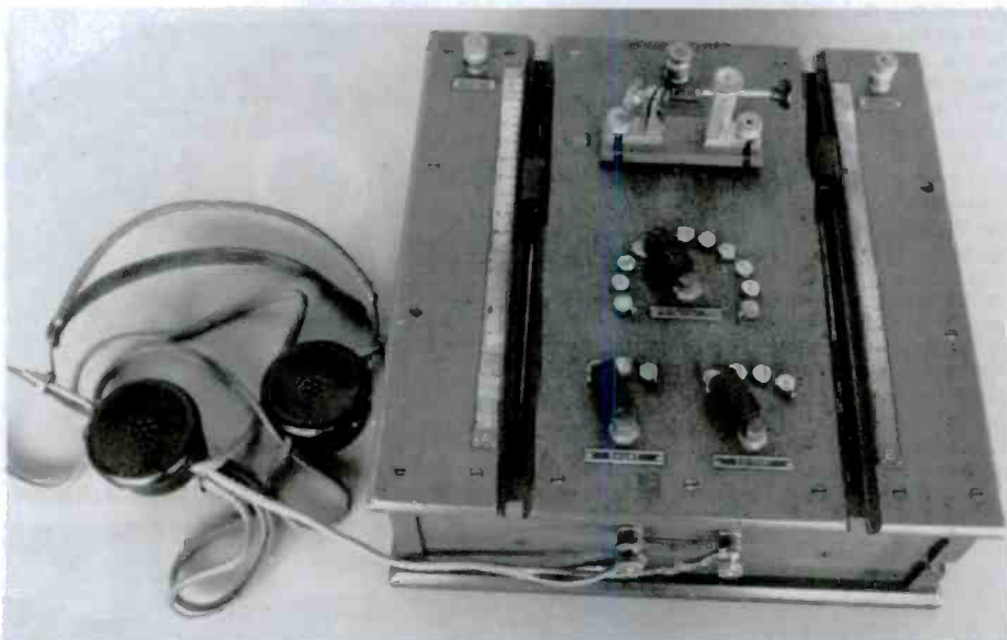
Figure 10. United Wireless Type D Tuner. This two-coil tuner (200-2000 meters) has two sliders on each coil. A Carborundum detector (seen at the rear) was included with an internal battery and tap switches to control the bias voltage. This particular set is about five percent larger than other existing Type D tuners and may be the de Forest version that preceded United Wireless. This 1910 version is part of the Perham collection, now at the Foothill Museum.
