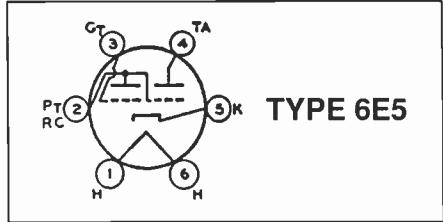
Figure 1. The Type 6E5 tuning eye tube base diagram. ("RCA Receiving Tube Manual," 1963, page 245.)
