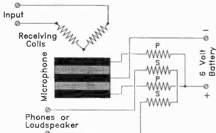
Figure 2. Circuit diagram of the Brown microphone amplifier.
