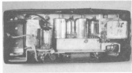
Rear interior view of the RCA Model BP-10 production radio. Compare this set with Figure 2 of the prototype portable.
