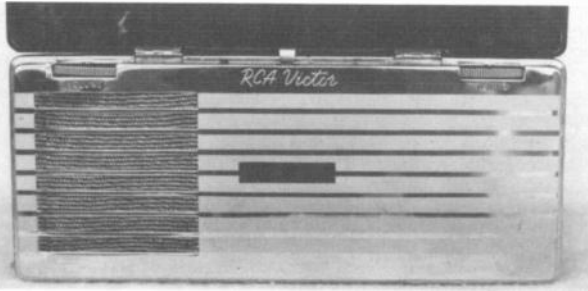
Figure 1. The front panel of the RCA prototype set with the cover lid in the open position. Note the spring-loaded cover tab above the RCA label. This activates the on/off switch when the lid is opened and closed. The metal case is 3" x 3.5" x 9", with black leatherette covering, plastic lid and chrome-plated front. A carrying strap once attached to one end of the case is now missing.
