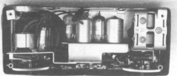
Figure 2. Rear interior view of the RCA portable prototype radio with the metal back cover removed.
