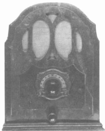
MIDGET CATHEDRAL - This Steinite is thirteen inches tall. It has a two-tone effect finish on the cabinet. It is a five-tube TRF receiver. The dial escutcheon is identical to that of the Avalon cathedral that appeared on the October 1987 cover of A.R.C. Steinite was made by the Warwick Mfg. Co. which produced some 40 trade names including Beverly, Clarion, Steinite and possibly Avalon. (Curtis P. Schreiber - Rochester, MN)
