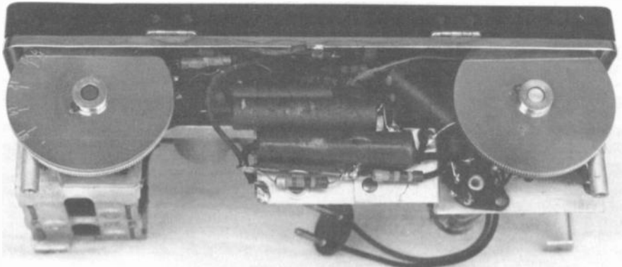
Figure 3. Another interior view of the RCA portable showing the tuning and volume control wheels.
