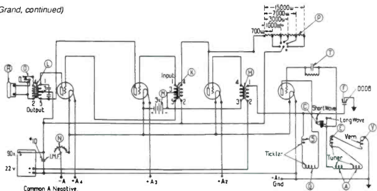
Figure 7. Schematic diagram of the Radiola Grand. (From the RCA Service Notes for 1923-1928)
