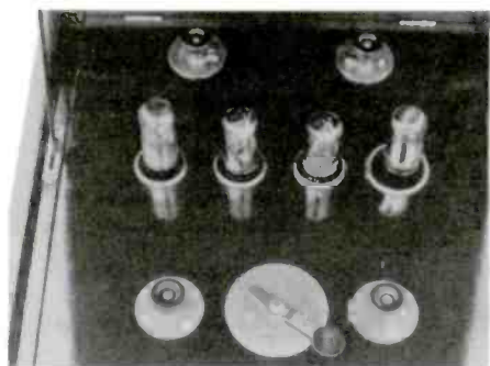
Figure 2. The Radiola Grand instrument panel showing the controls and four Type 864 tubes.
