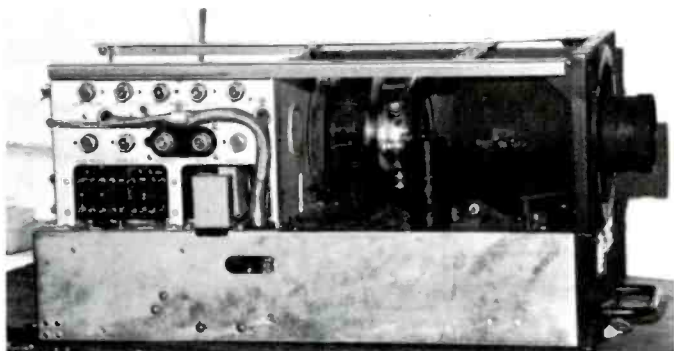
Figure 1. Side view of the BC-1211 camera unit.
