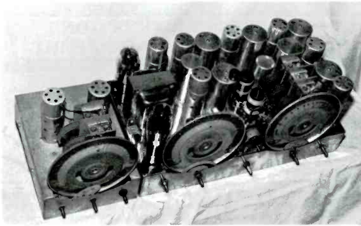
Figure 2. Chassis for the Patterson PR-10 receiver and Patterson pre-selector.
