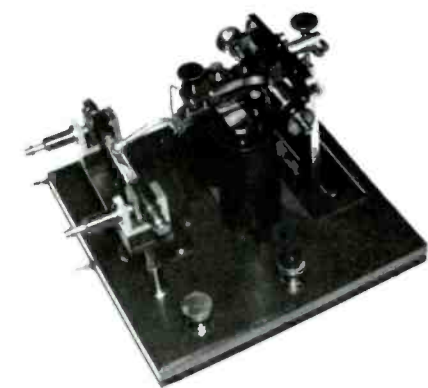
1905 Branley Coherer detector. The coherer is on the left with the tapper above. Contest entry by Andre Chompert.
