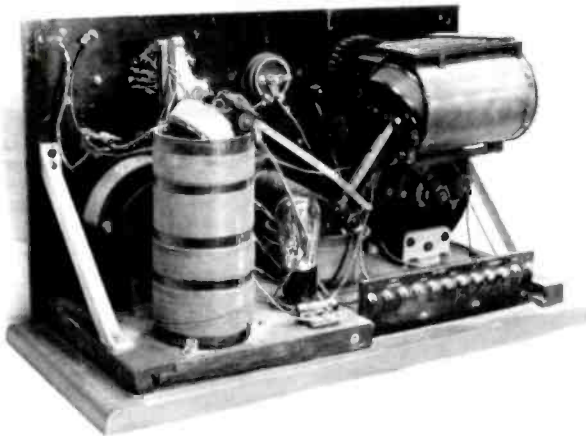
Figure 3. The restored Model 106D chassis showing the location of the detector tube installed by RCA.
