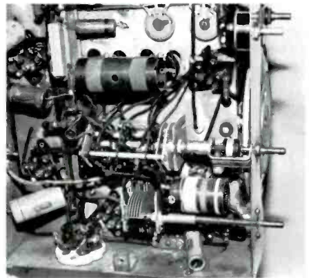
Figure 3. Underside of the Patterson PR-10 receiver showing the tuning mechanism and uncoated wire-wound coils.
