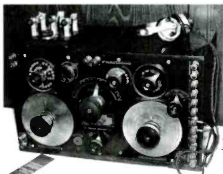
Marconi CM 294C, manufactured in 1917, with a triple detector. Contest entry by Larry Babcock.
