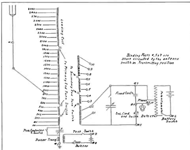
Figure 4. Schematic diagram of the earlier Type 106 Receiver using only a crystal type detector for reception.
