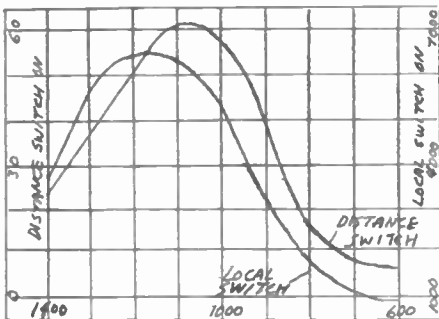
Figure 3. Sensitivity in uv/m. Left scale is the distance switch on; right scale, local switch on.
