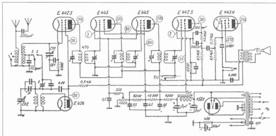
Figure 2. Circuit diagram for the The Lemouzy Super Resonance receiver.
