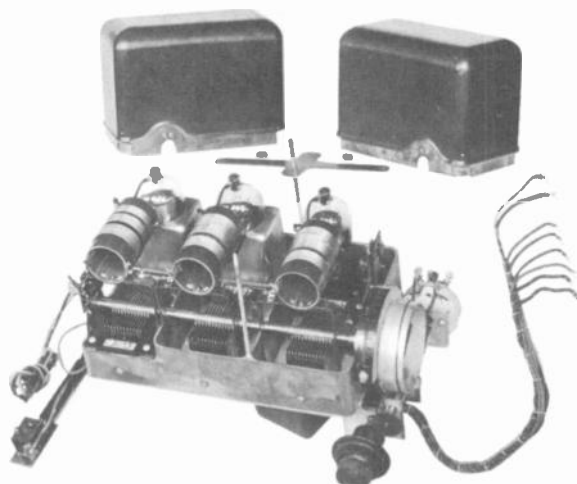
Figure 6. The receiver assembly which uses three UY-224s.
