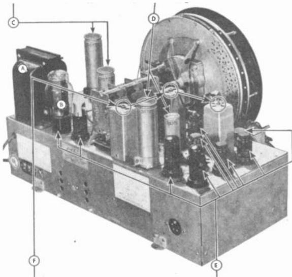
Figure 4. A typical AC radio chassis with the filter capacitors, power transformer, and rectifier tube identified. A = power transformer, B = rectifier tube, C & D = filter capacitors, E = tubes, F = IF transformers.
