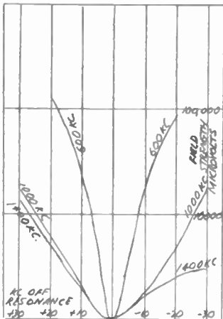
Figure 2. Selectivity in uv/m as a function of KC off resonance.
