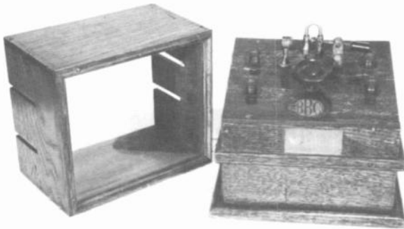
Figure 5. The Walmore Set. The manufacturer is unknown. The date is circa 1923. The case is made of oak, and has a removable glass cover. The panel slopes to the front. A removable u-shaped link can be replaced by a loading coil for other frequencies one might wish to tune. Size is 7'' \times 6\frac{1}{4}'' \times 7\frac{1}{4}'' .
