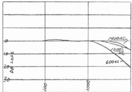
Figure 4. Frequency response curve, DB loss as a function of frequency in cycles.
