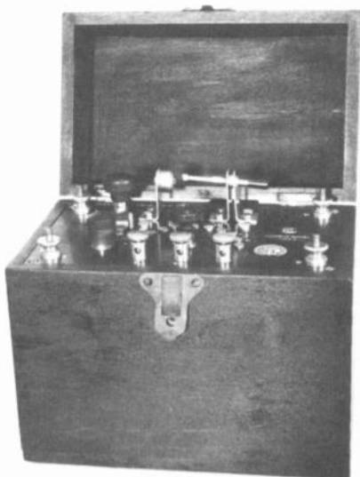
Figure 1. Ediswan Model 1923B. G.P.O. #433. Manufactured by Ediswan, 123 Queen Victoria St., London. First produced in 1923, it has a mahogany case with a lid. It is 4 3/4" x 8" x 7 1/2". The knob on the left front holds spare crystals. It has tapped inductance tuning. An ad in the October 10, 1923, issue of "The Wireless World and Radio Review" said, "Clear and loud reception is readily obtained over a range of 25 miles under favourable conditions. Receives on wavelengths between 200 and 500 metres." It cost £3.7.6 including headphones.
