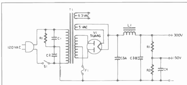
Figure 2. Vacuum-tube full-wave power supply using a power transformer.
