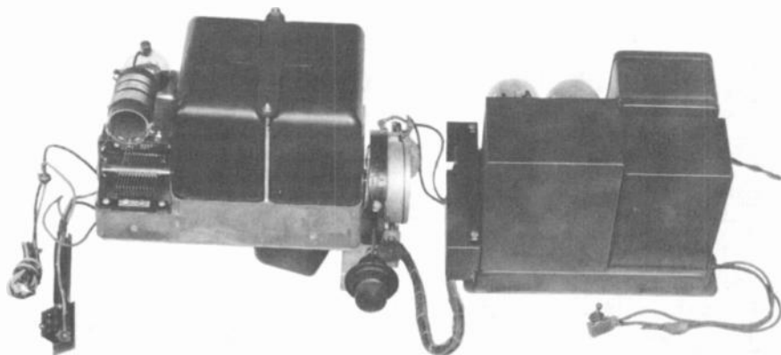
Figure 7. On the left is the three-tube receiver assembly. On the right is the power unit which includes the power supply (UX-280) and the audio output amplifier (UX-245).
