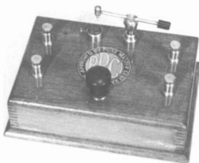
Figure 2. Master Junior. G.P.O. #899. It was manufactured by Master Radio, 30 Rosamond St. East, All Saints, Manchester. The date is 1923-24. The small simple case is finished in a light tan color. It receives 250 to 600 meters. It has an open detector. The size is 5 1/4" x 4" x 1 1/2". It has slide coil tuning. It cost £0.7.6.
