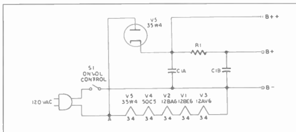
Figure 3. Universal AC-DC power supply, not using a power transformer.
