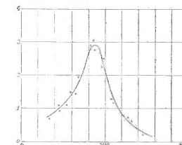
Figure 4. Spark gap length vs. sphere spacing. (Hertz, pg. 45)
