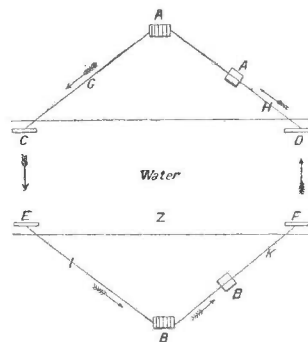
Figure 1. Signals were transmitted from A to B using water at points C-E and D-F to complete the circuit. Distance Z had to be much greater than the width of the river. (Fahie, pg. 26)
