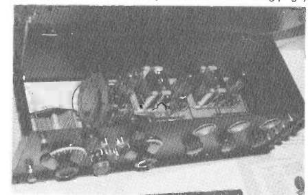
An outstanding example of a Reinartz receiver in the old equipment contest entered by Ross Smith.
