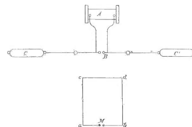
Figure 3. Hertz's experimental apparatus. (Hertz, pg. 40)
