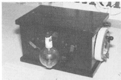
A spherical audion, displayed in a DeForest RJ-4, a contest entry by Larry Babcock.
