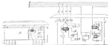
Figure 2. Signals were transmitted between the wires strung above the trains and the conductors "a" in the roof of the trains. (Fahie, pg 105)
