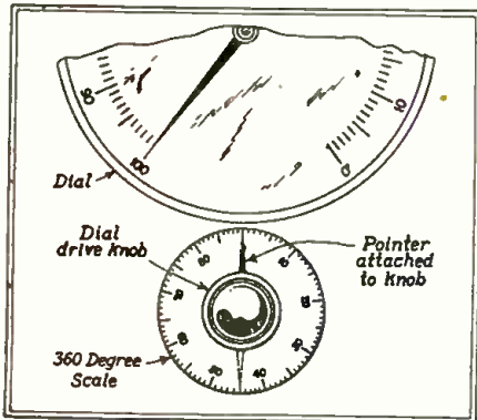
Simple means of adding band-spread to an all-wave tuning dial.
