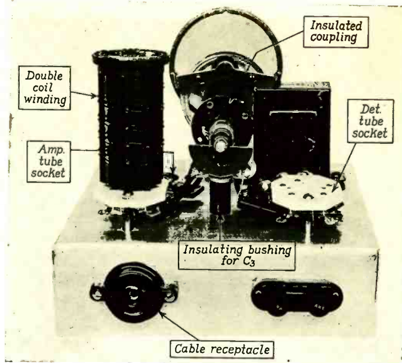
Fig. 3. Rear view of the completed receiver.
