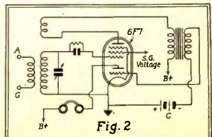
Using the 6F7 as a regenerative detector and reflexed audio amplifier.
