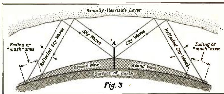
Fig. 3 Sky waves are reflected or refracted by the ionized layer in the upper atmosphere and, so, return to earth. Note the areas where they interfere with the weak ground waves.
