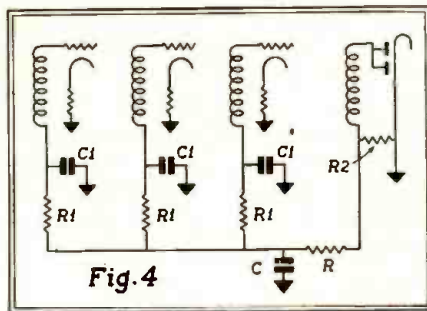
Typical avc system suitable for short-wave receivers.
