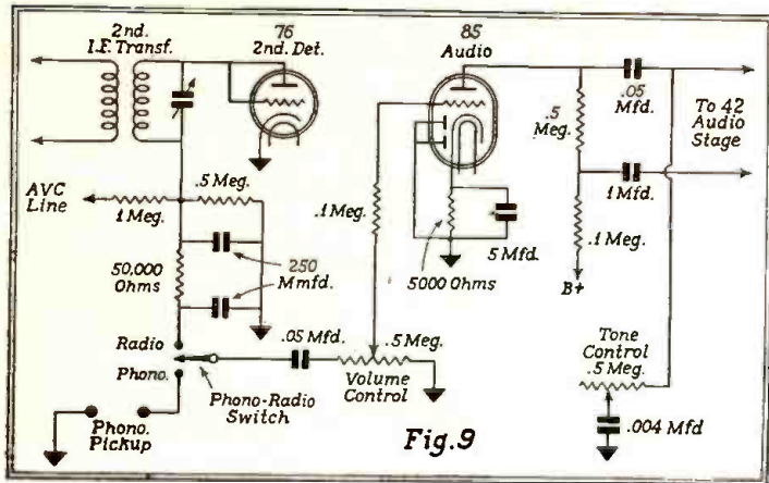
Second detector and first a-f circuit of the Lafayette Receiver, showing the AVC and phono connections.
