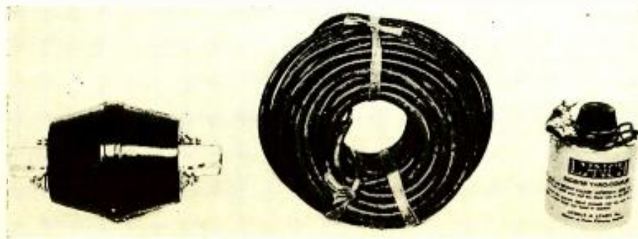
Fig. 5. The principal working units of an all-wave, noise-reducing antenna system: Antenna coupling transformer; heavy-duty, low-impedance transmission line; receiver coupling transformer with variable impedance adjuster.
