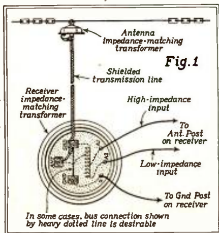
A noise-reducing aerial system expressly designed for broadcast reception.
