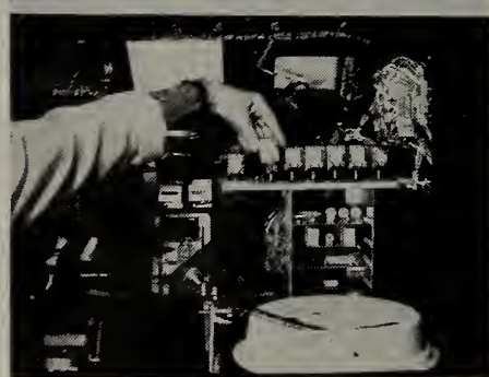
The top photo shows the plug-in photocell board that serves as the heart of the answer coding of Computer Quiz. Using this system, questions and related answers can never be separated. Bottom photo indicates one of 13 plug-in relays.
