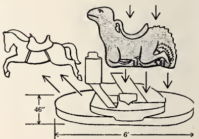
Southland DINOSAUR (Transfer of Removable Body)
