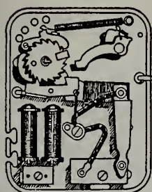
MAGAZINE SWITCH BOX ASSEMBLY
