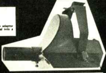
PROJECTOR LX-3 — A.B.S. antihot body — Quartz iodine-lamp v 24 w 150 — Incorporated transformer — Turbine-cooling — Interchangeable object-glass — Double condenser — Parabolic mirror — Antihot incorporated filter — Manual control of object-glass — Feeding v 220 Hz 50
