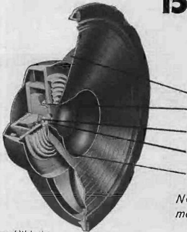
Cutaway of Wolverine Model LS15
