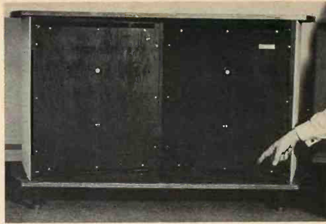
The backs of the two speaker systems comprising the Stereorama II form an angle, and the back-waves from the ports blend to form a center channel in a stereo setup.
