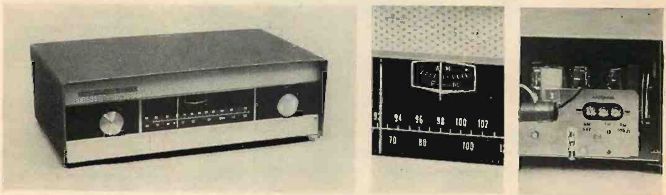
The General Electric FA-11 and FA-12 AM/FM tuners are available in either a gray or russet vinyl wrap-around. The face plate is rippled black and silver. Exceptionally "active" tuning meter makes spotting for either AM or FM signals a breeze. Only complaint we had with the structural design was in the location of the antenna input terminals (far right photo). Unless considerable care is exercised, stray strands of lead-in wire tend to short out antenna input to surrounding close fitting metal bracket.
